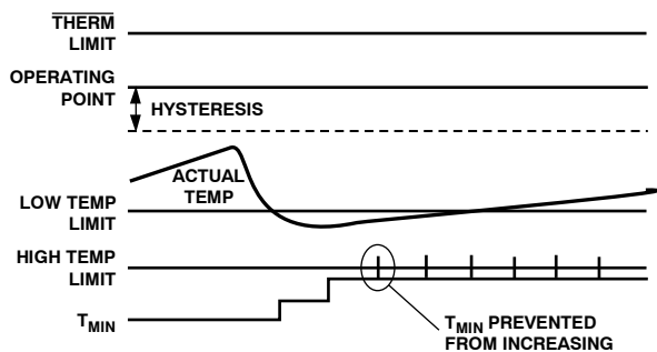
Figure 75. T_{MIN} Adjustments Limited by the High Temperature Limit
