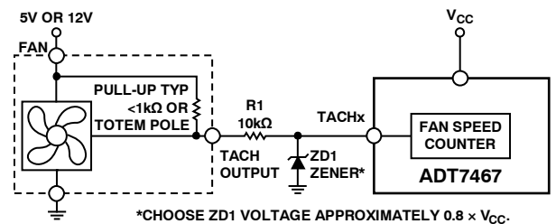
Figure 44. Fan with Strong TACH Pull-Up to >V_{CC} or Totem-Pole Output,
