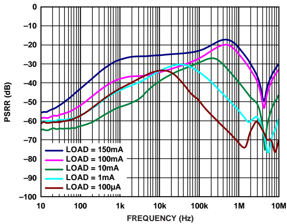
Figure 21. Power Supply Rejection Ratio vs. Frequency Various Output Voltages and Load Currents, V_{OUT} = 2.5V , V_{IN} = 3.0V
