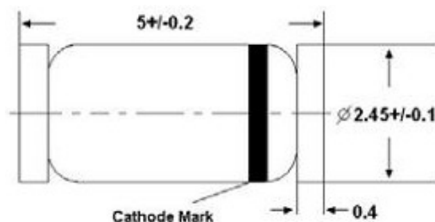
Glass Case MELF Dimensions in mm
