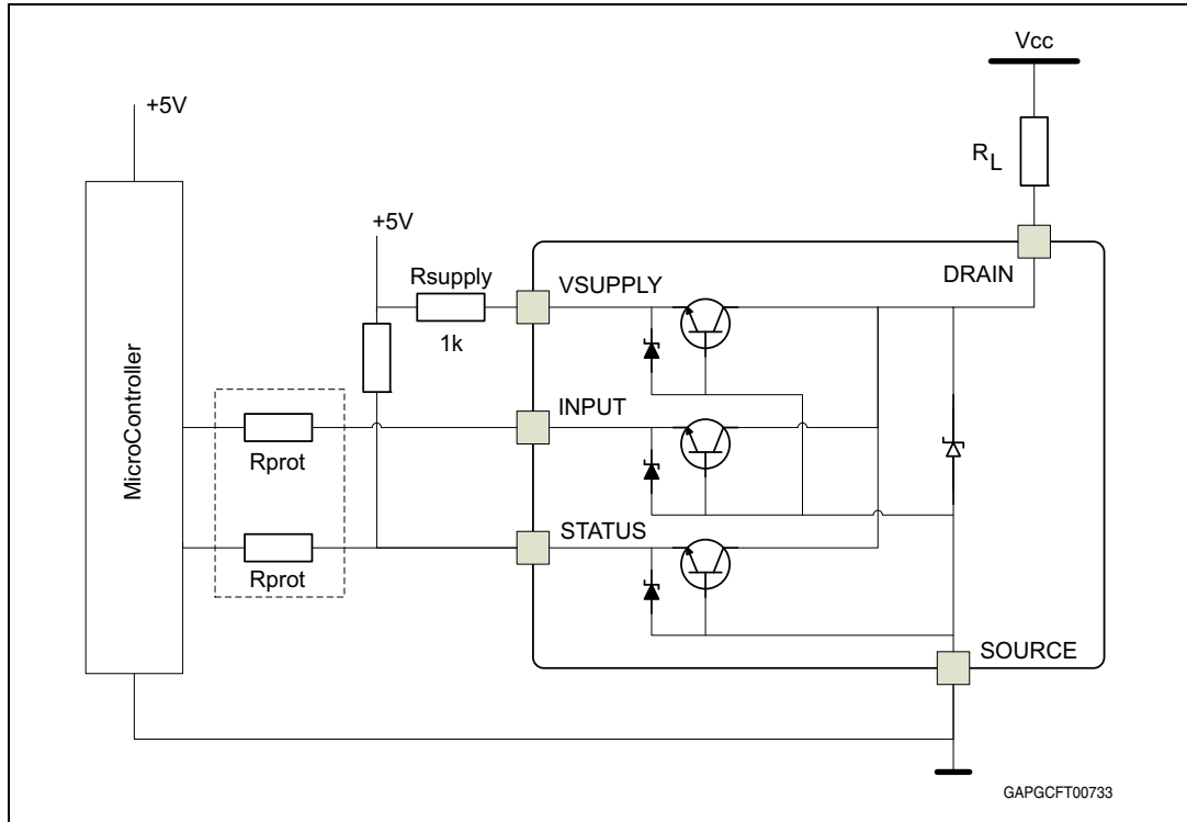
Figure 5. Application schematic
