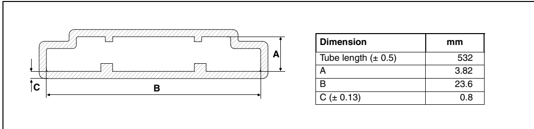
Figure 46. MultiPowerSO-30 tube shipment (no suffix)
