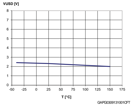
Figure 24: Undervoltage shutdown
