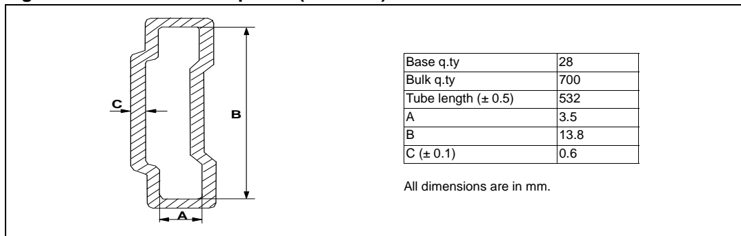
Figure 37. SO-28 tube shipment (no suffix)
