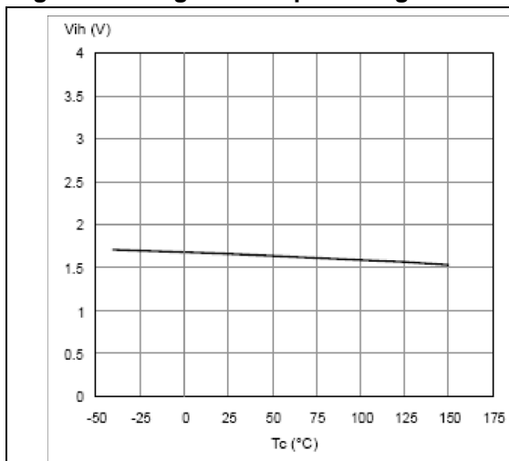
Figure 10. High-level input voltage
