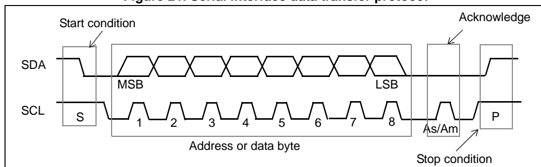
Figure 21. Serial interface data transfer protocol
