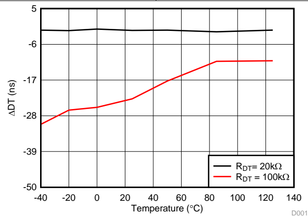
Figure 25. Dead Time vs. Temperature (with R DT = 20 kΩ and 100 kΩ)
