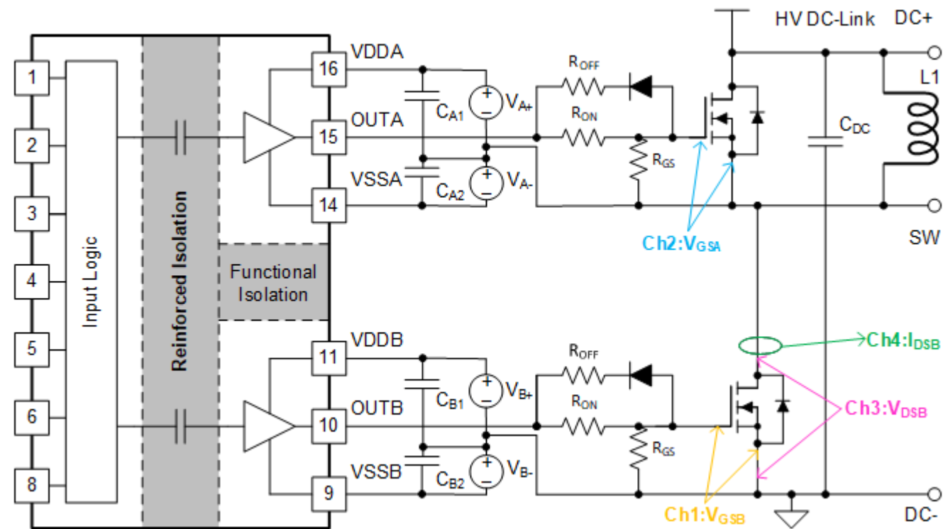
Figure 42. Bench Test Circuit with SiC MOSFET Switching
