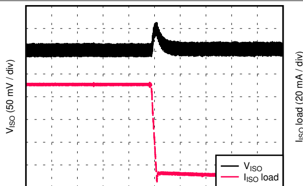
Figure 38. V_{ISO} Load Transient Response, 90% to 10% Load Step, 5.0-V Input, 5.4-V Output
