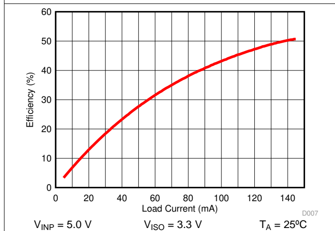
Figure 14. Power Supply Efficiency vs Load Current ( I_{ISO} )
