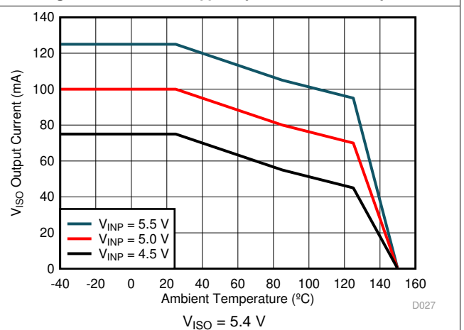
Figure 9. Maximum V_{ISO} Output Current vs. Temperature
