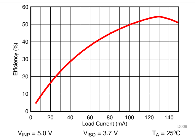
Figure 15. Power Supply Efficiency vs Load Current ( I_{ISO} )
