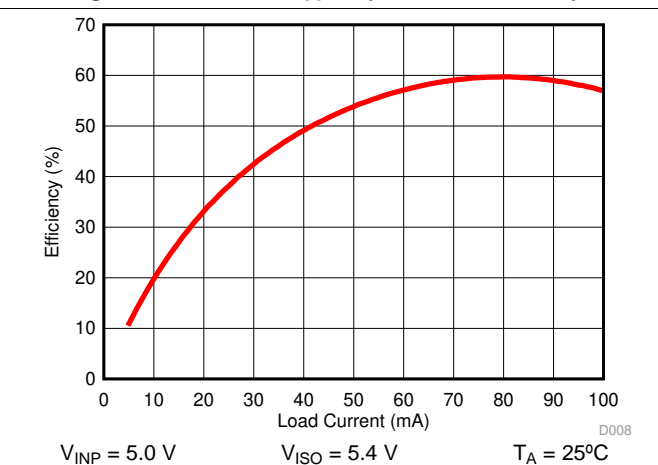
Figure 13. Power Supply Efficiency vs Load Current ( I_{ISO} )
