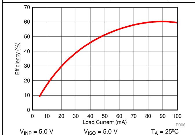
Figure 12. Power Supply Efficiency vs Load Current ( I_{ISO} )
