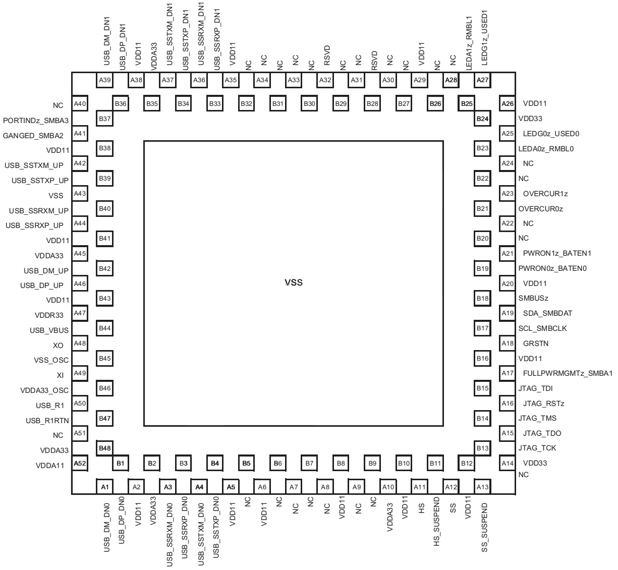
TUSB8020ARKM (Top View)
