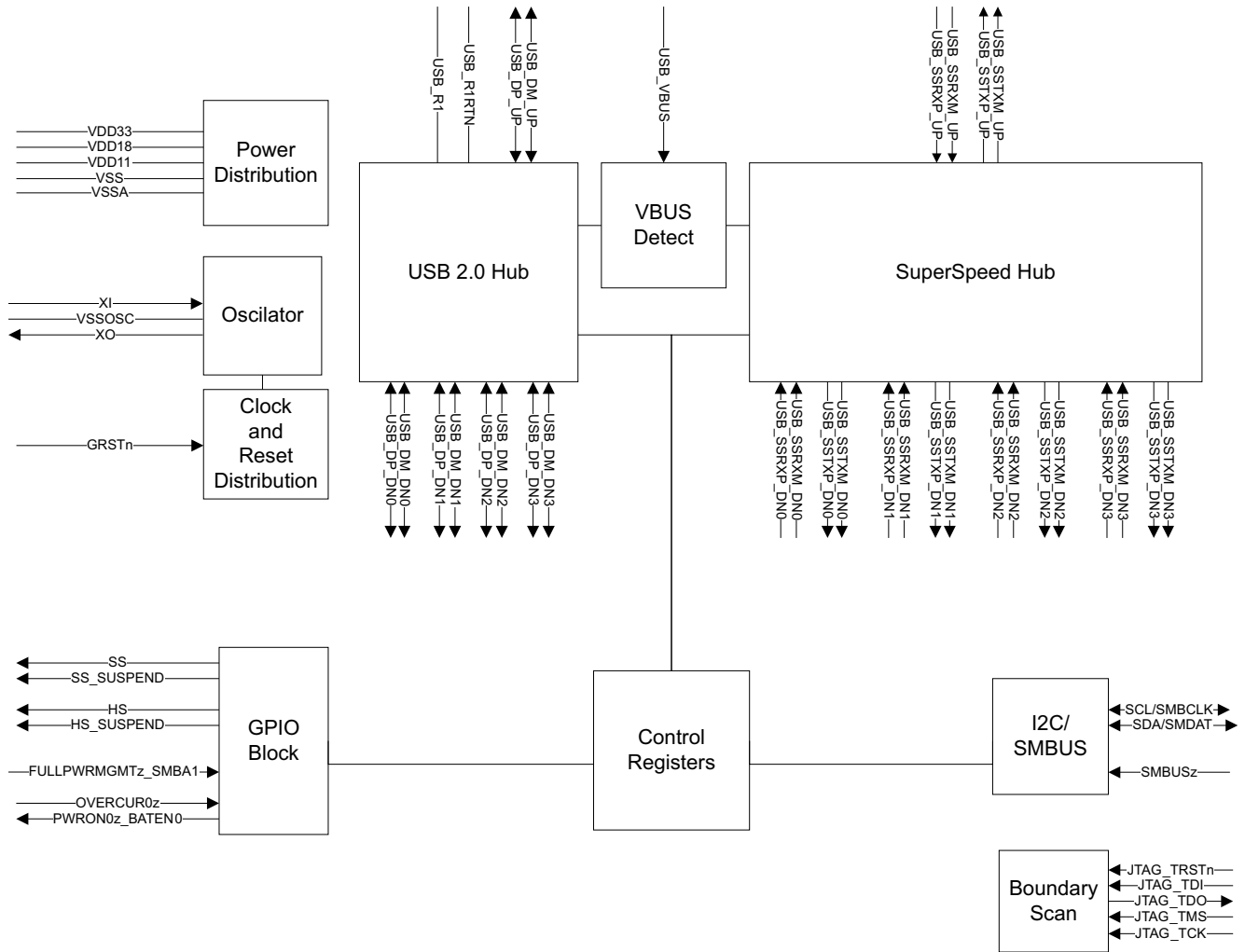
Figure 1-3. TUSB8040APFP Functional Block Diagram
