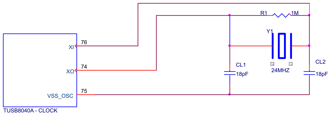
Figure 4-1. TUSB8040A Clock
