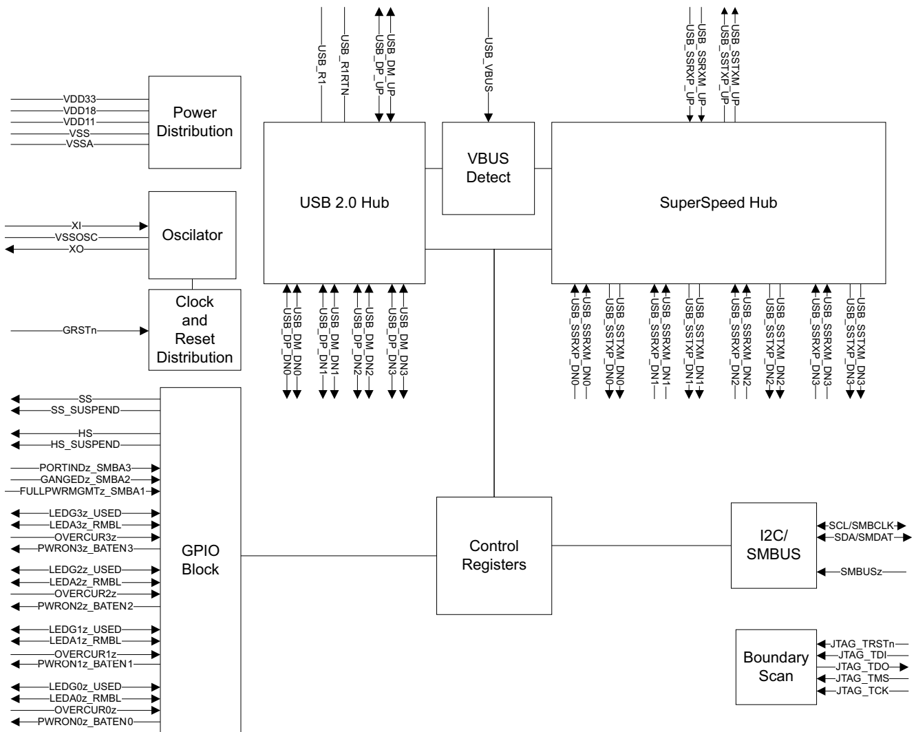
Figure 1-2. TUSB8040ARKM Functional Block Diagram
