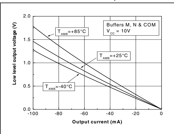
Figure 19. Voltage output low ( V_{OL} ) vs. output current - Buffers M, N & COM
