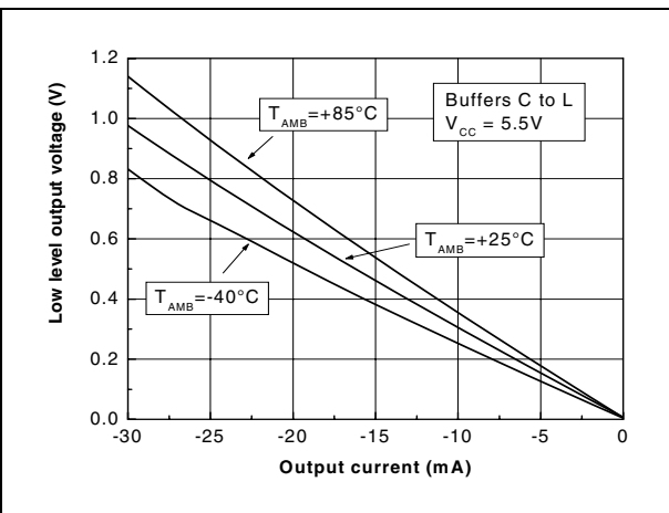
Figure 15. Voltage output low ( V_{OL} ) vs. output current - Buffers C to L
