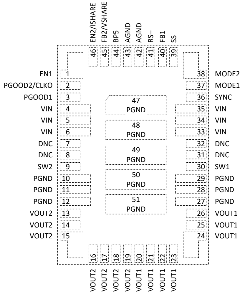
Figure 5-1. 51-Pin, QFN Package (Top View)
