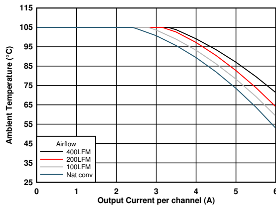
Figure 6-10. Safe Operating Area (VOUT = 1.8 V)
