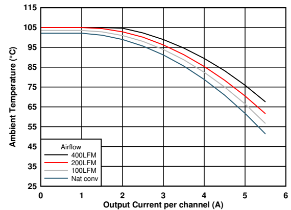
Figure 6-4. Safe Operating Area (VOUT = 1.8 V)
