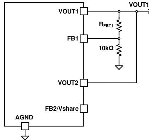
Figure 7-2. Single Device, Current Sharing
