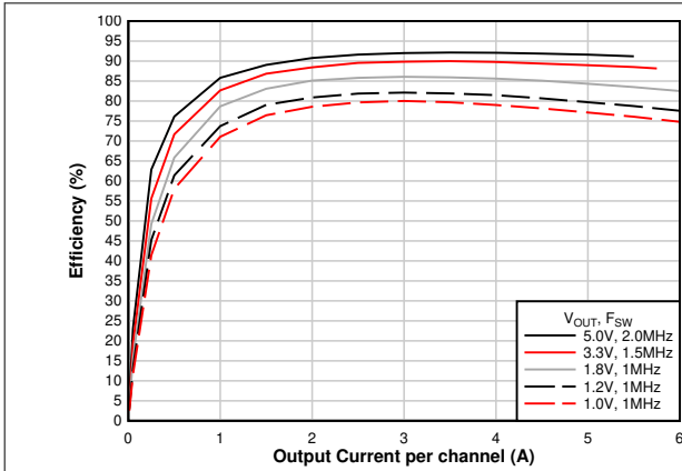
Figure 6-1. Efficiency vs Output Current
