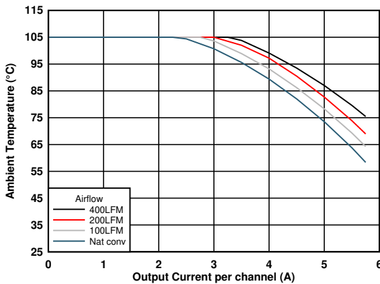
Figure 6-3. Safe Operating Area (VOUT = 1.2 V)
