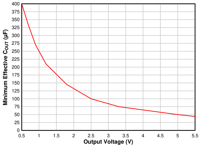
Figure 7-6. Minimum Required Output Capacitance (per Phase)
