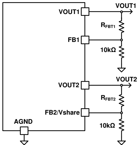
Figure 7-1. Single Device, Dual Output
