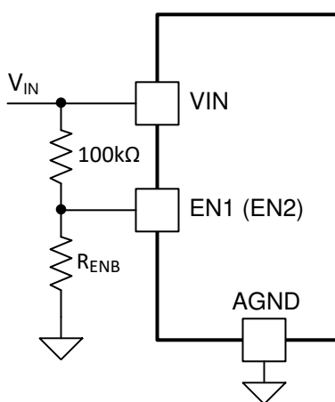
Figure 7-7. Enable ON/OFF Control
