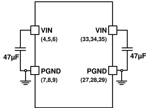
Figure 7-5. Input Capacitors Pin Connections
