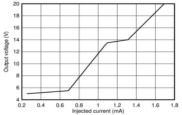
Figure 6-32. Output Voltage vs Injected Current
