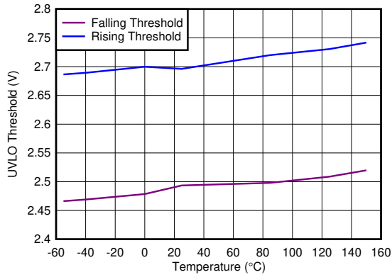
Figure 6-31. Undervoltage Lockout (UVLO) Threshold vs Temperature
