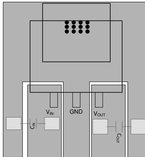
Figure 10-1. KVU Package Fixed Output
