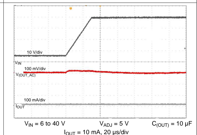
Figure 18. 6- to 40-V Line Transient
