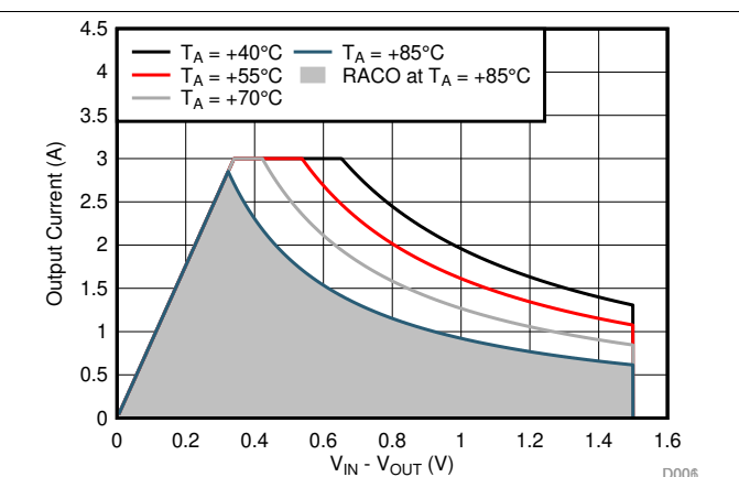
Figure 68. Recommended Area for Continuous Operation for V_{OUT} = 5\text{ V}
