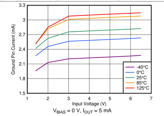
Figure 32. Ground Pin Current vs Input Voltage
