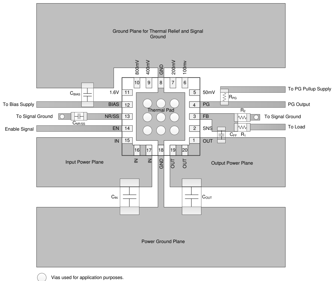
Figure 72. Example Layout
