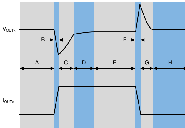
Figure 57. Load Transient Waveform
