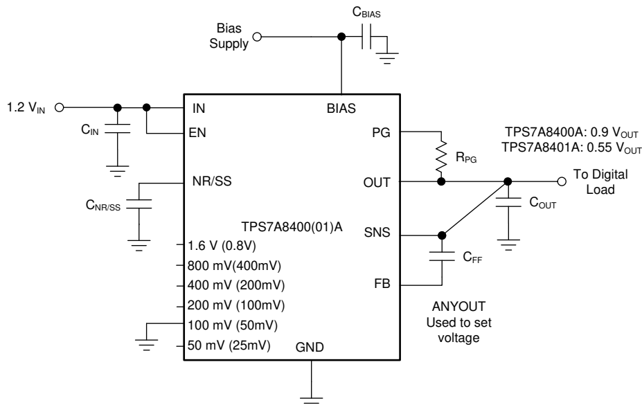
Figure 51. ANY-OUT Configuration Circuit (0.9-V, 0.55-V Output with Bias)
