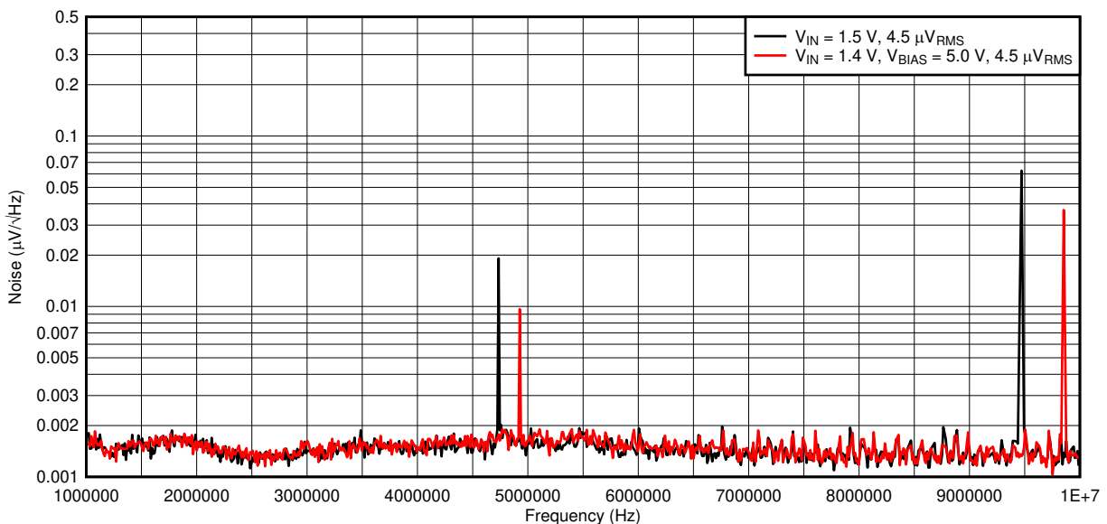
Figure 56. Charge Pump Noise
