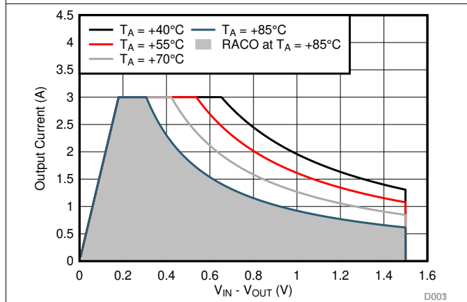
Figure 65. Recommended Area for Continuous Operation for V_{OUT} = 1.8\text{ V}
