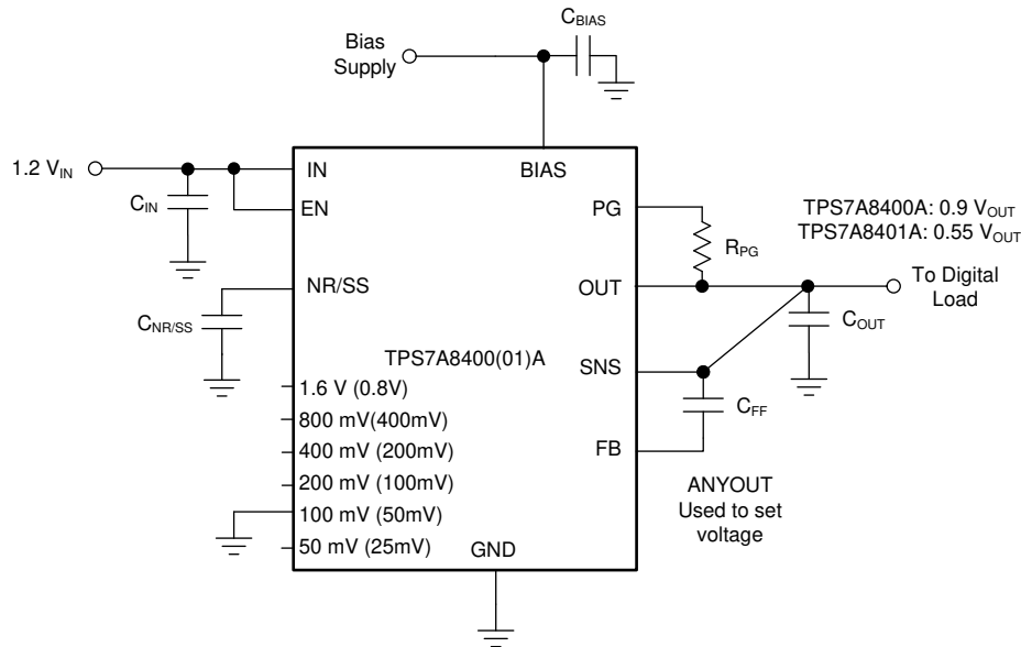
Figure 69. TPS7A84A Typical Application
