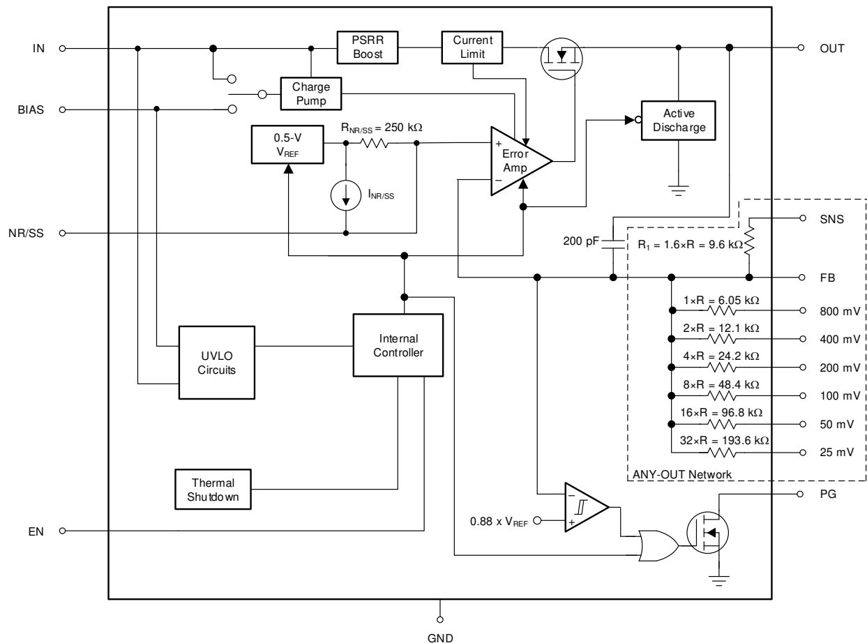
Figure 44. TPS7A8401A Block Diagram
