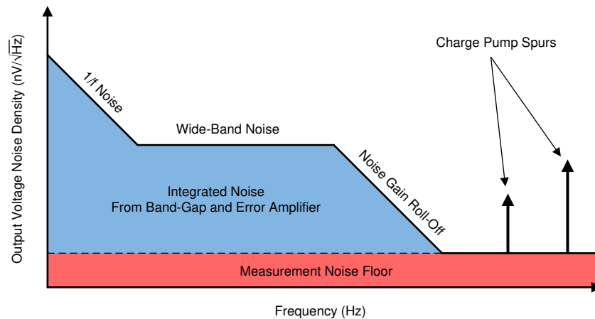
Figure 55. Output Voltage Noise Diagram
