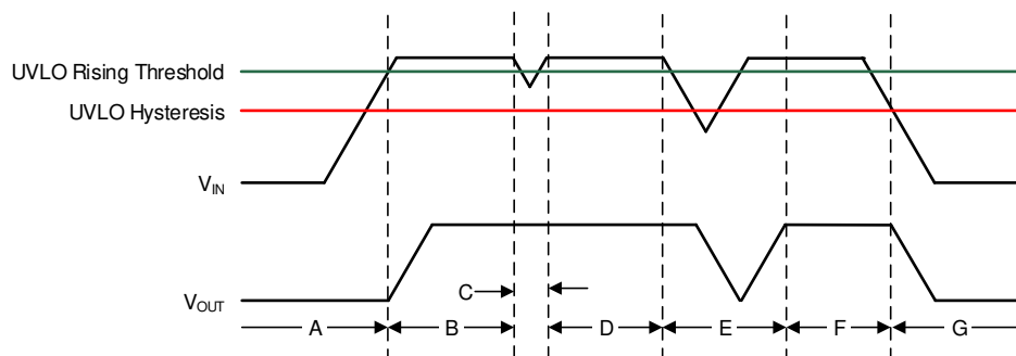
Figure 52. Typical UVLO Operation
