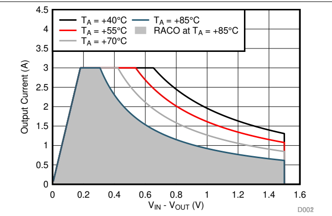
Figure 64. Recommended Area for Continuous Operation for V_{OUT} = 1.2\text{ V}
