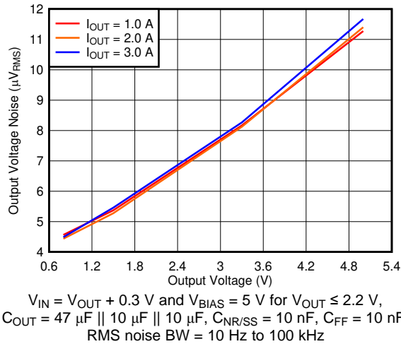
Figure 9. Output Voltage Noise vs Output Voltage
