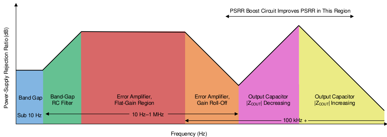
Figure 54. Power-Supply Rejection Ratio Diagram
