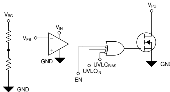
Figure 48. Simplified PG Circuit
