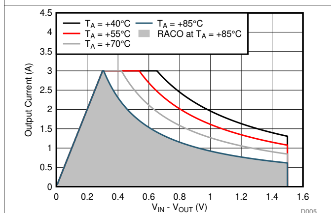
Figure 67. Recommended Area for Continuous Operation for V_{OUT} = 3.3\text{ V}
