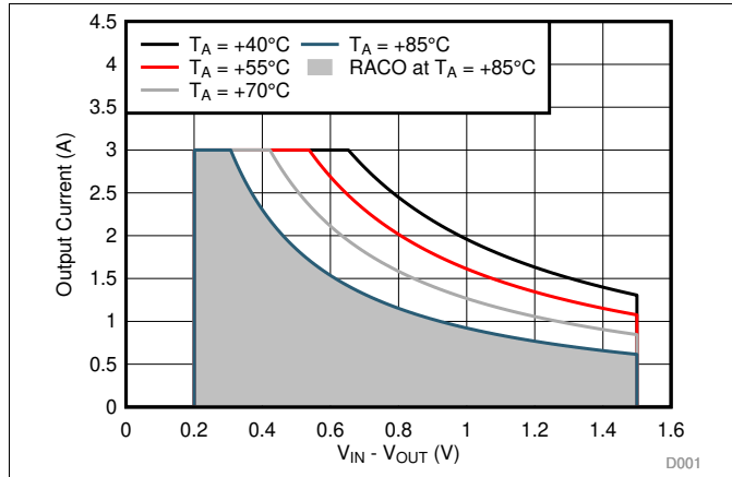
Figure 63. Recommended Area for Continuous Operation for V_{OUT} = 0.9\text{ V}
