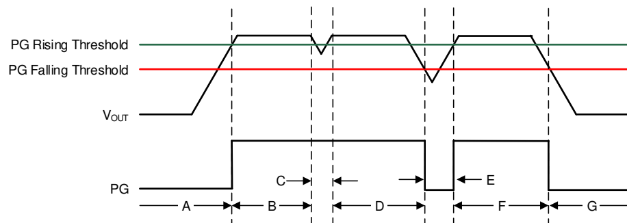
Figure 53. Typical PG Operation
