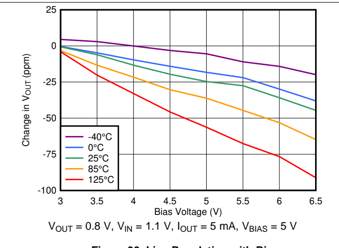
Figure 30. Line Regulation with Bias
