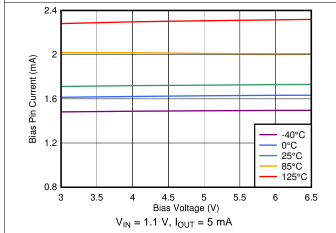
Figure 33. Bias Pin Current vs Bias Voltage
