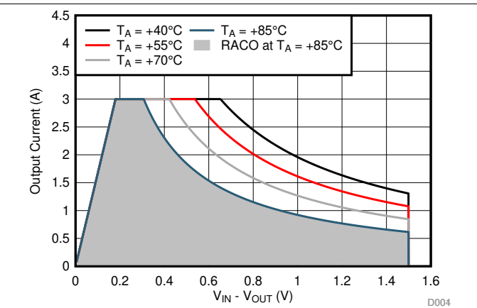
Figure 66. Recommended Area for Continuous Operation for V_{OUT} = 2.5\text{ V}
