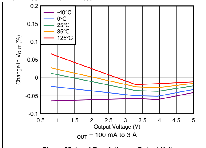
Figure 25. Load Regulation vs Output Voltage
