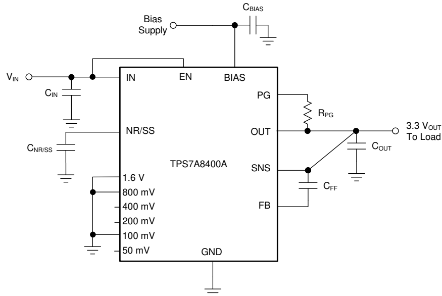
Figure 50. ANY-OUT Configuration Circuit (TPS7A8400A) (3.3-V Output, No External Bias)
