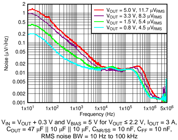
Figure 10. Output Noise vs Frequency and Output Voltage
