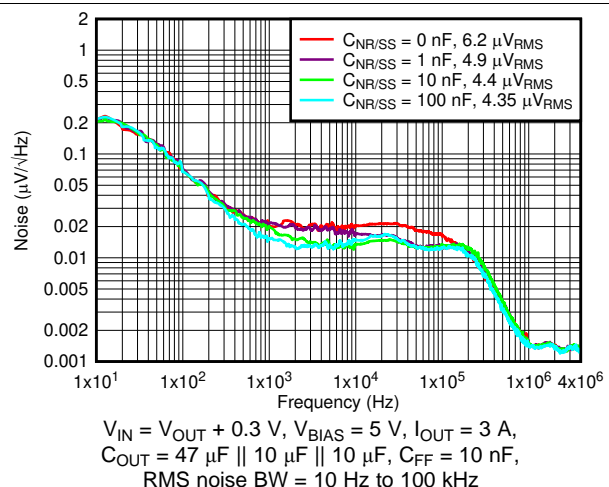
Figure 12. Output Noise vs Frequency and C_{NR/SS}
