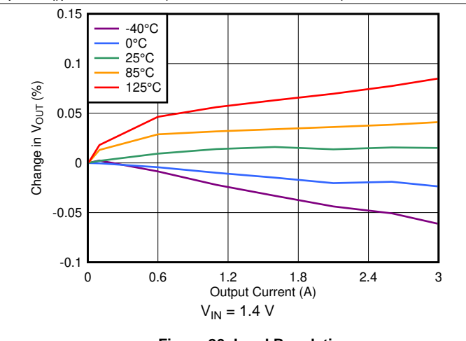
Figure 26. Load Regulation
