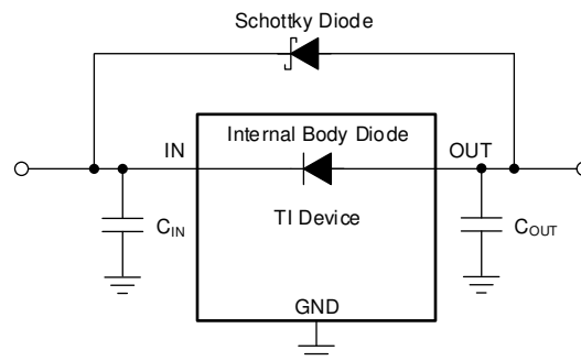
Figure 61. Example Circuit for Reverse Current Protection Using a Schottky Diode
