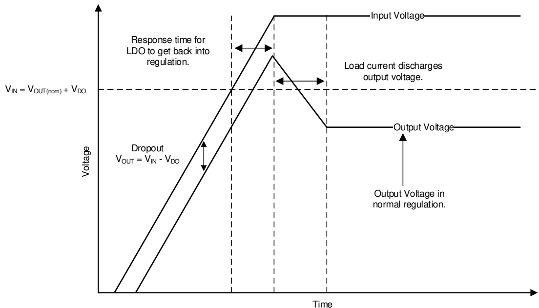
Figure 60. Start-Up Into Dropout
