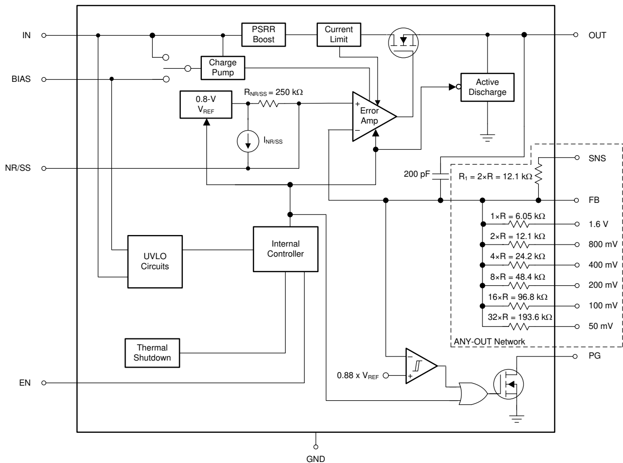
Figure 43. TPS7A8400A Block Diagram
