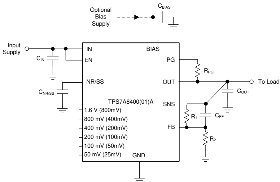
Figure 49. Adjustable Operation
