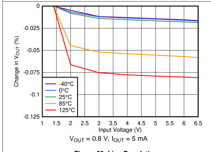
Figure 29. Line Regulation
