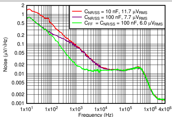
Figure 14. Output Noise at 5-V Output
