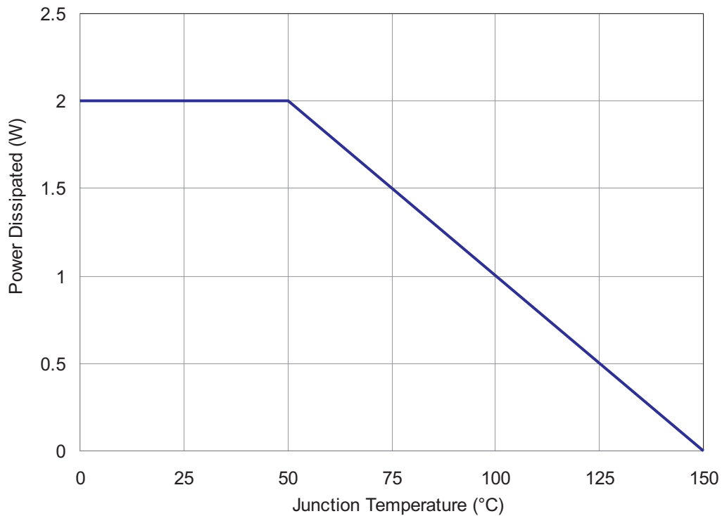
Figure 36. Power Derating Curve
