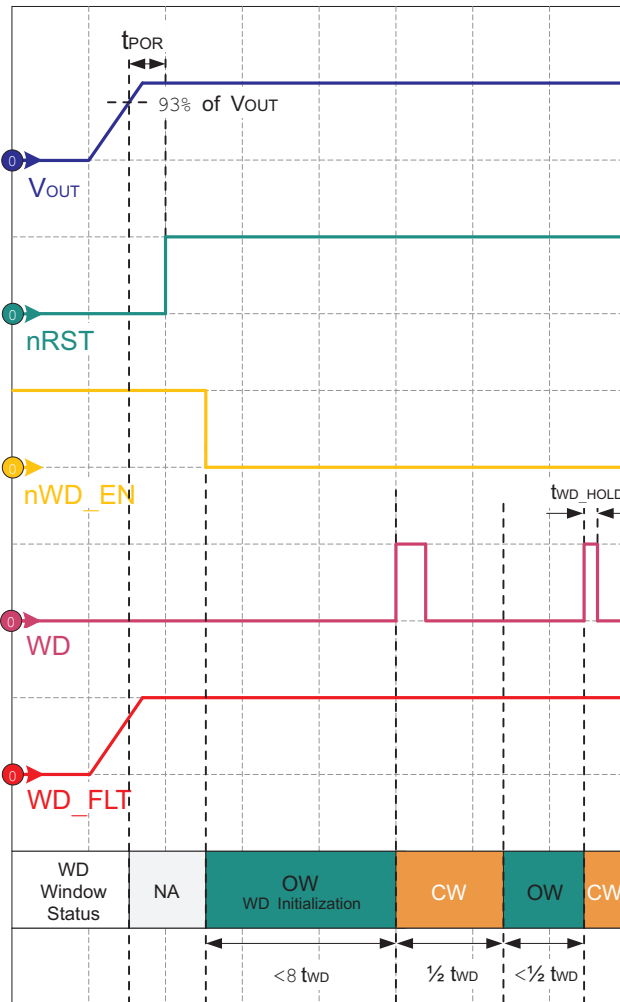
Figure 23. Power Up, Initialization, and Normal Operation for TPS7A63xx-Q1
