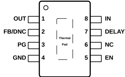
DGN Package 8-Pin HVSSOP With Exposed Thermal Pad Top View
