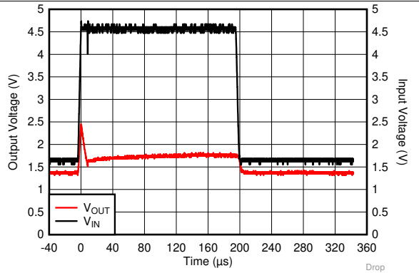
V_{OUT} = 1.8\text{ V} , I_{OUT} = 100\text{ mA} , C_{OUT} = 1\ \mu\text{F} , slew rate = 1\text{ V}/\mu\text{s}
