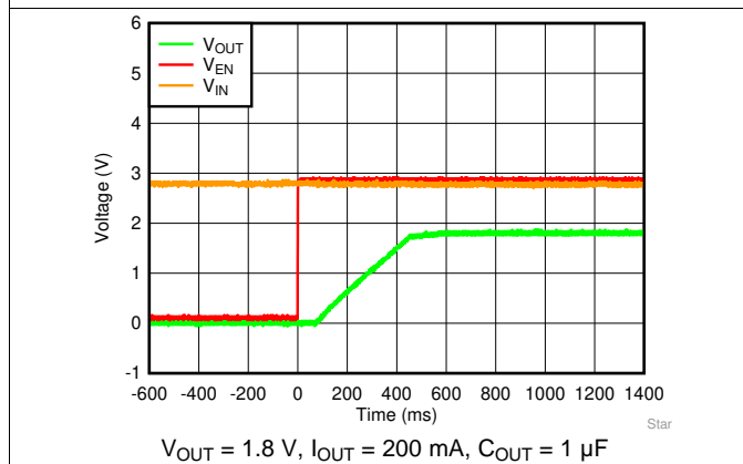
Figure 53. Startup With V_{EN} After V_{IN}
