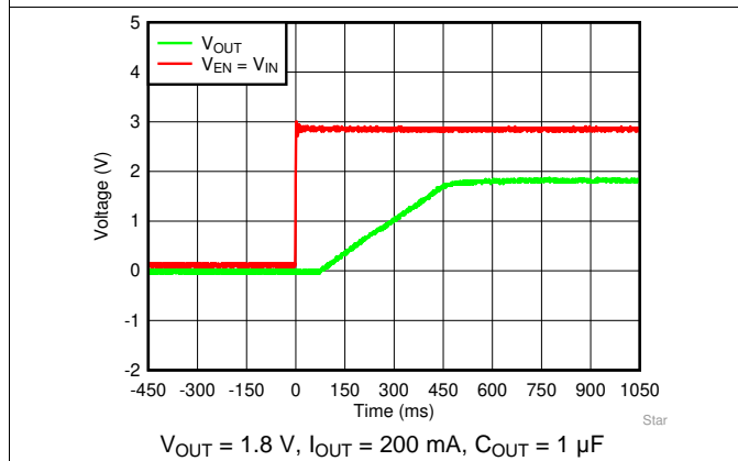
Figure 51. Startup With V_{EN} = V_{IN}
