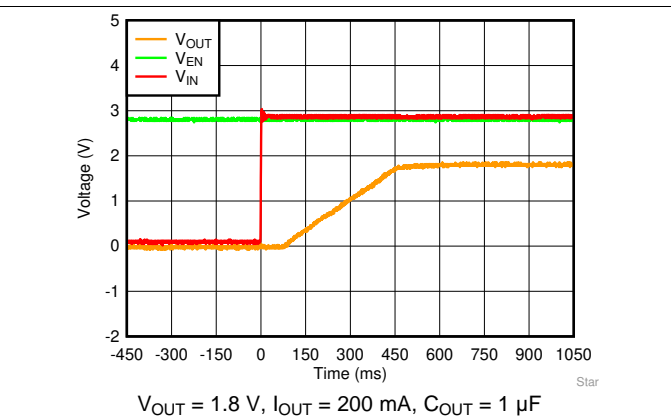
Figure 52. Startup With V_{EN} Before V_{IN}
