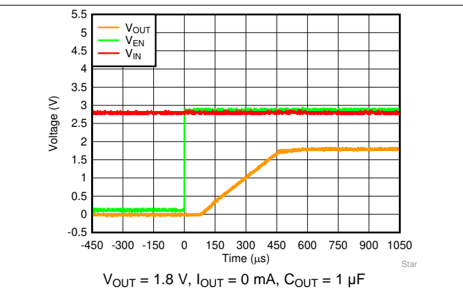
Figure 54. Startup With V_{EN} After V_{IN}
