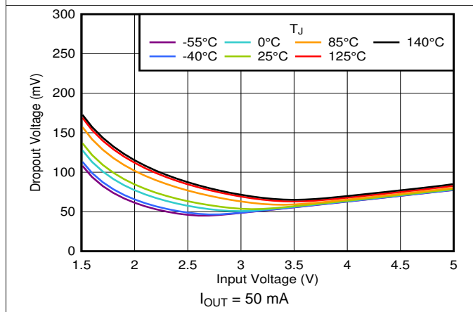
Figure 35. Dropout vs V_{IN} and Temperature
