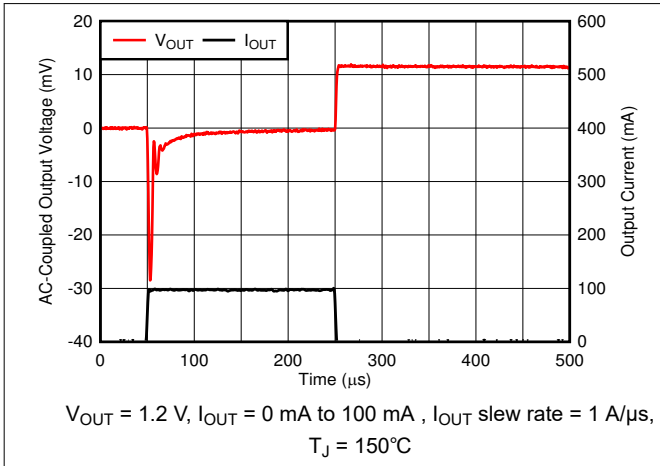
Figure 6-49. Load Transient
