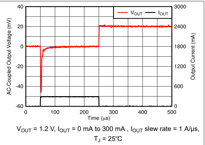
Figure 6-50. Load Transient
