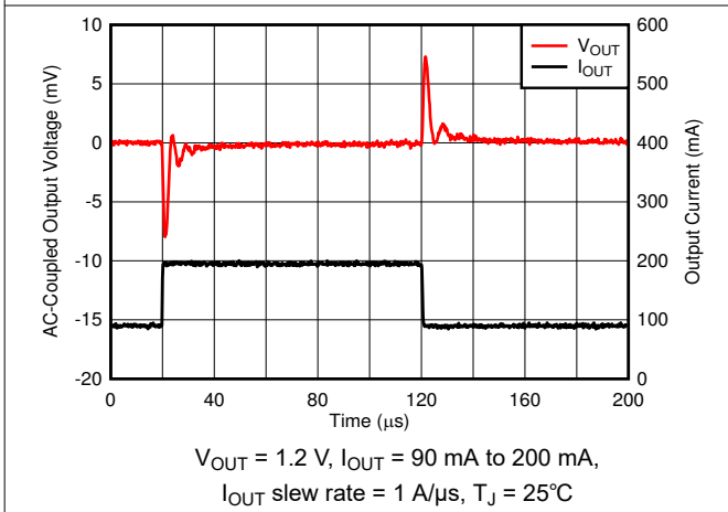
Figure 6-53. Load Transient
