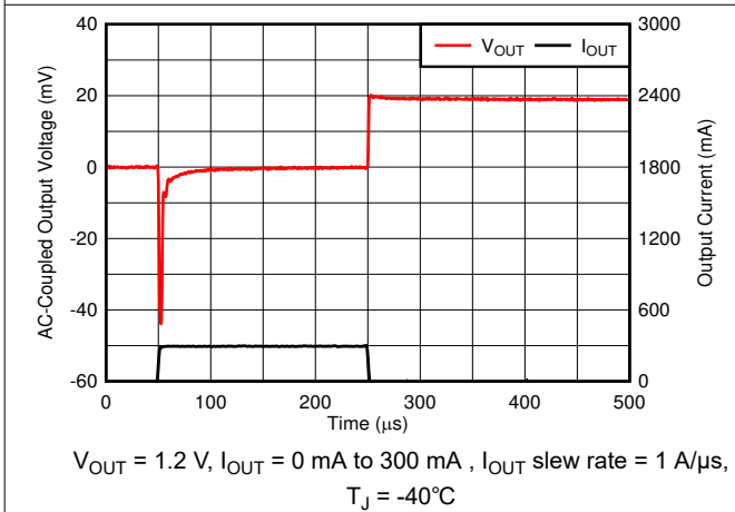
Figure 6-51. Load Transient
