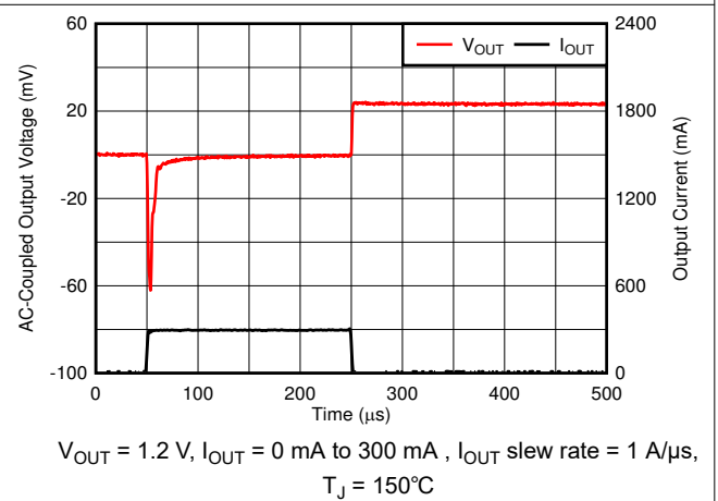
Figure 6-52. Load Transient
