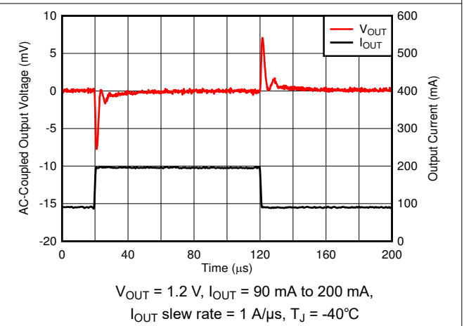
Figure 6-54. Load Transient
