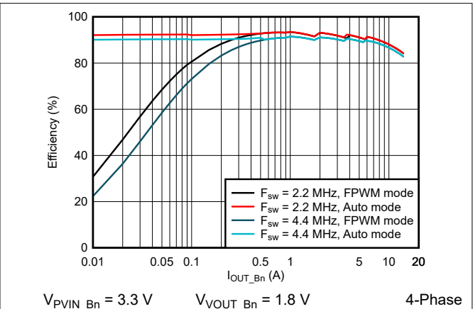
Figure 9-5. BUCK Efficiency with Fsw = 2.2 MHz or 4.4 MHz
