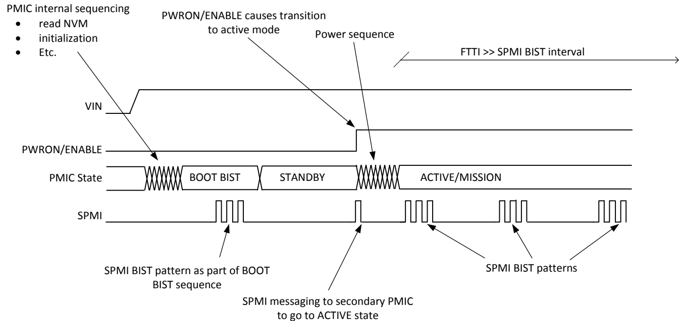
Figure 8-50. SPMI-BIST Operation
