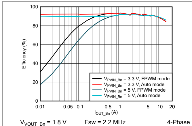
Figure 9-4. BUCK Efficiency at 3.3 V or 5 V Input Voltage
