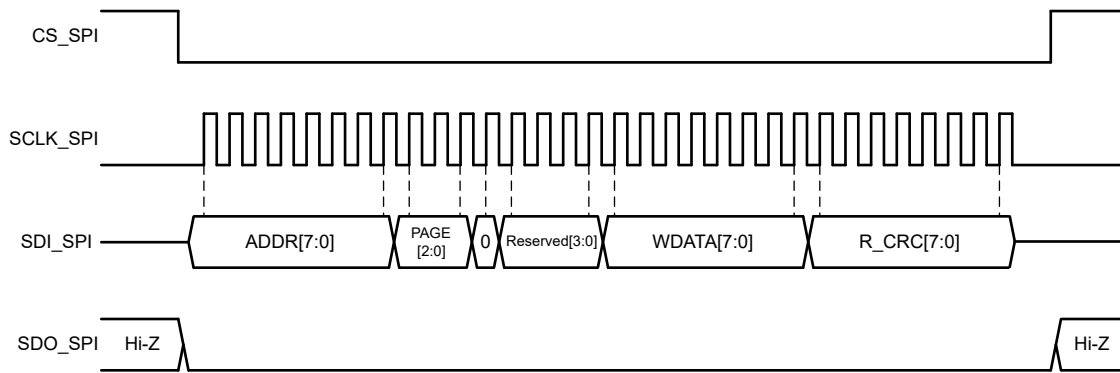
Figure 8-62. SPI Write Cycle with CRC
