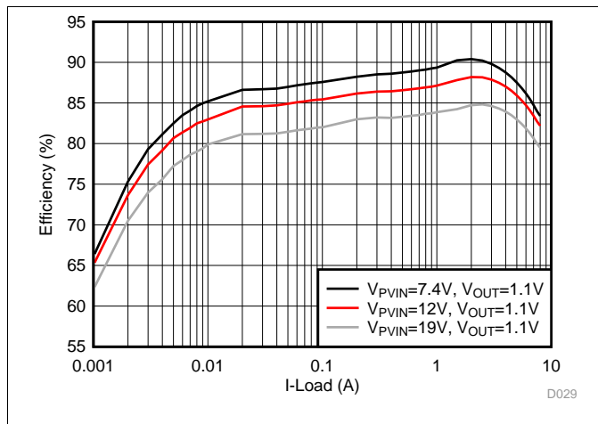
Figure 33. VDD2 Efficiency Curve, V_{OUT} = 1.1 V
