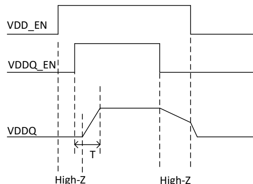
Figure 30. Power Sequence, VDDQ vs VDDQ_EN
