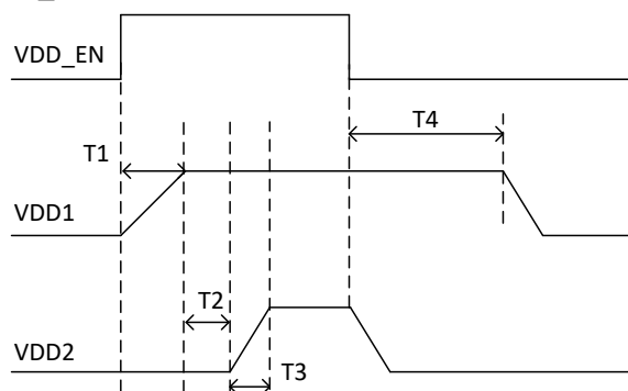
Figure 29. Power Sequence, VDD1 and VDD2 vs VDD_EN
