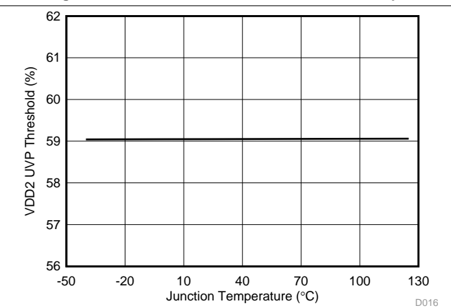
Figure 14. VDD2 UVP Threshold vs Junction Temperature
