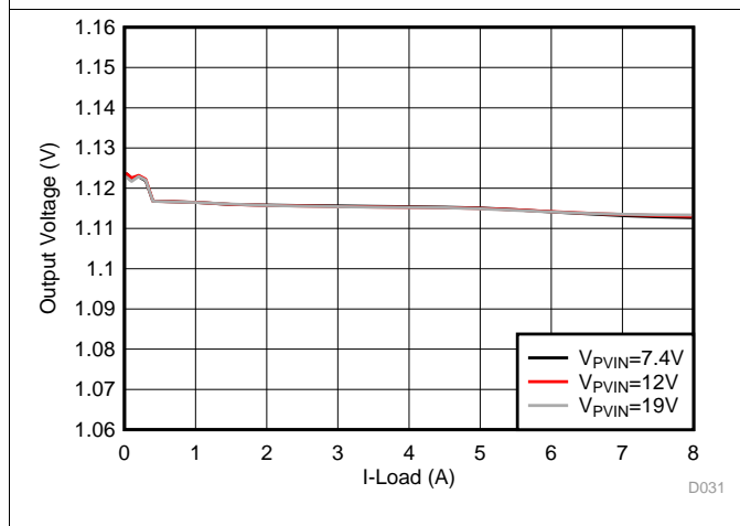
Figure 35. VDD2 Load Regulation, V_{OUT} = 1.1 V
