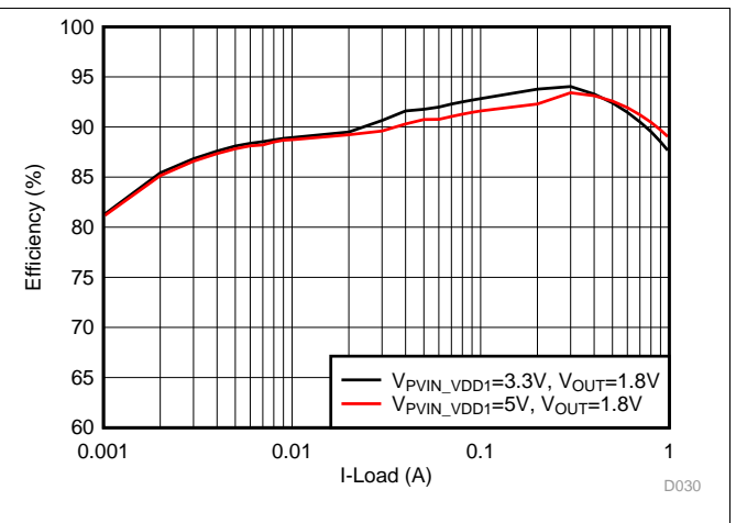
Figure 34. VDD1 Efficiency Curve, V_{OUT} = 1.8 V
