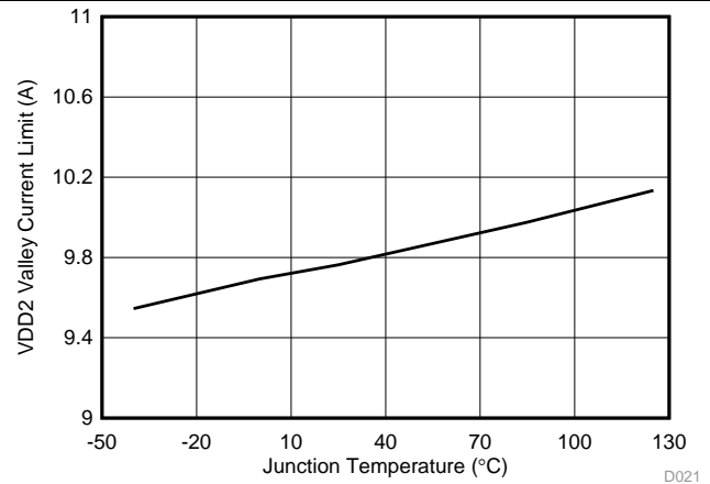
Figure 20. VDD2 Valley Current Limit vs Junction Temperature
