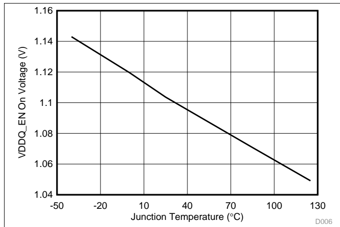
Figure 7. Enable On Voltage (VDDQ_EN) vs Junction Temperature
