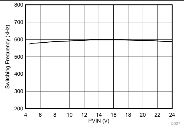
Figure 24. VDD2 Switching Frequency vs Input Voltage
