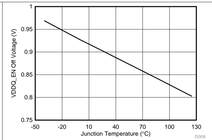
Figure 8. Enable Off Voltage (VDDQ_EN) vs Junction Temperature
