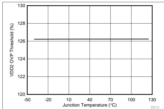
Figure 13. VDD2 OVP Threshold vs Junction Temperature
