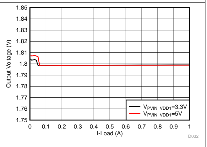
Figure 36. VDD1 Load Regulation, V_{OUT} = 1.8 V
