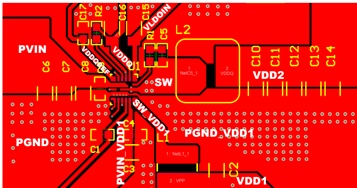
Figure 61. Top-Side Layout
