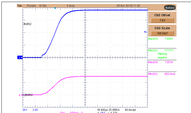
Figure 31. BUCK3 Start-Up V_{OUT} = 7.5\text{ V}, 0.7\text{ A}
