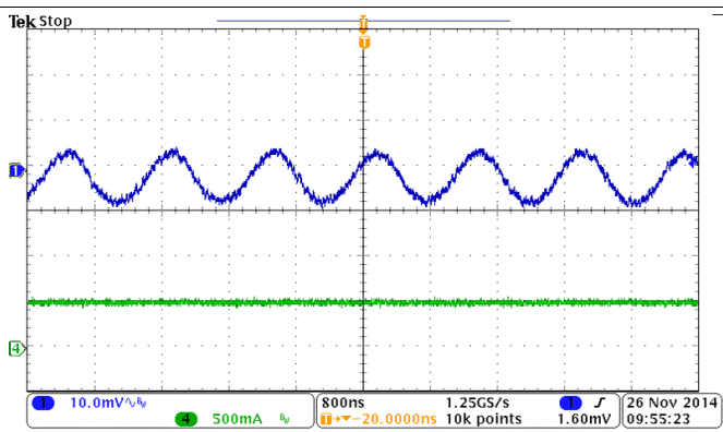
Figure 32. BUCK3 Ripple V_{OUT} = 7.5\text{ V}, 0.5\text{ A}, f_{SW} = 800\text{ kHz} 10 mV/div
