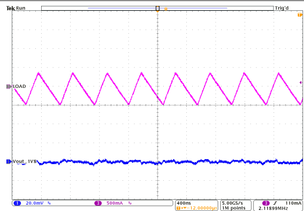
Figure 9-34. PSM Operation
