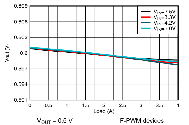
Figure 9-6. Load Regulation
