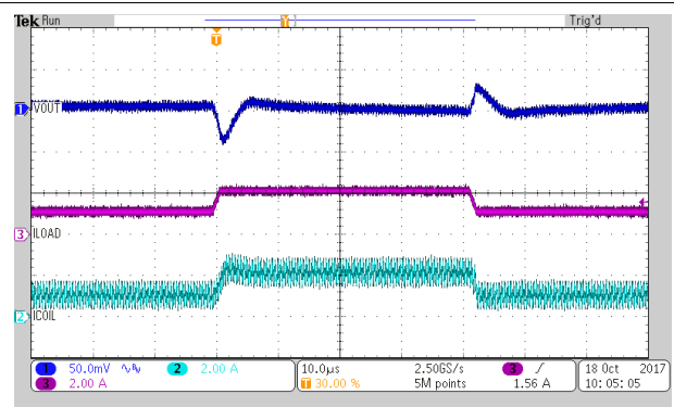
I_{OUT} = 1 \text{ A to } 2 \text{ A} TPS62825A/6A/7A
