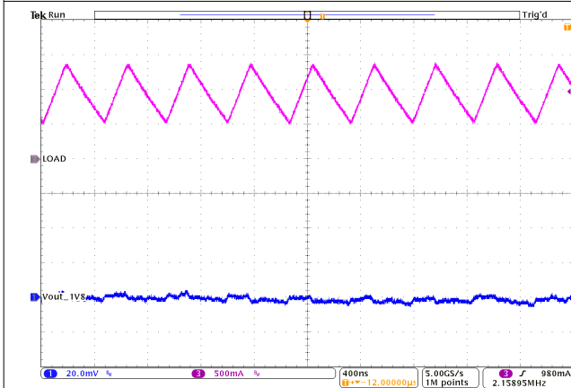
Figure 9-33. PWM Operation
