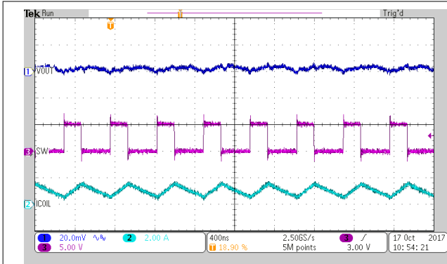
Figure 9-33. PWM Operation
