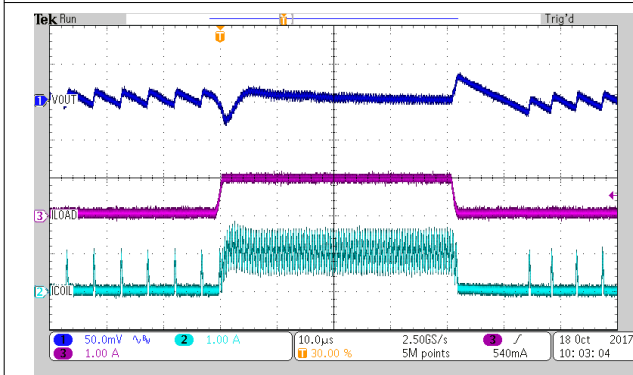
I_{OUT} = 0.05 \text{ A to } 1 \text{ A} TPS62824A/5A/6A/7A
