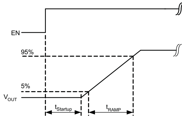
Figure 27. Soft Start
