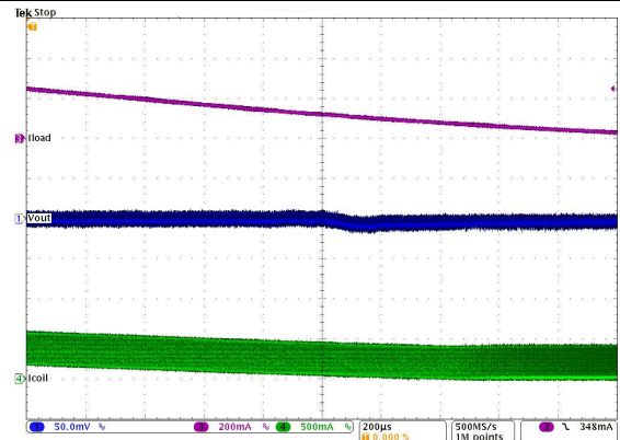
Figure 19. Maximum Output Current
