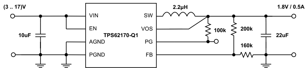
Figure 34. 1.8-V/0.5-A Power Supply
