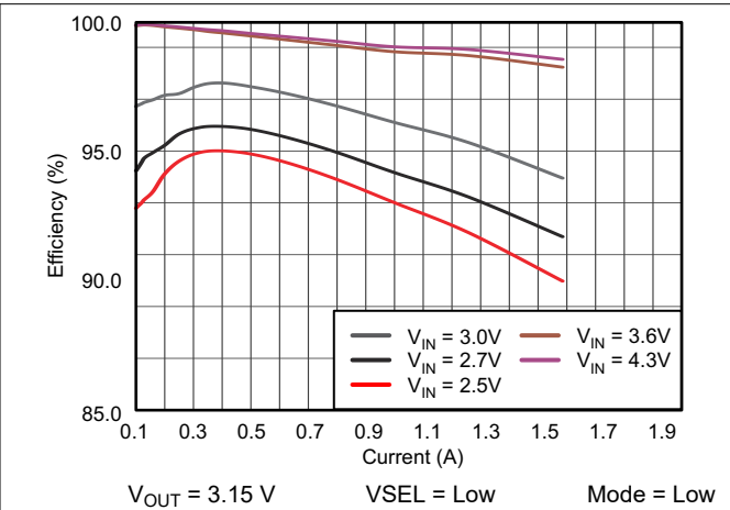
Figure 10-3. TPS61281D Efficiency vs Output Current
