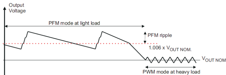
Figure 9-3. Power-Save Mode Ripple
