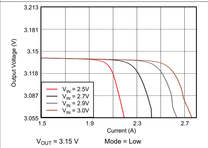
Figure 10-7. TPS61281D DC Output Voltage vs Output Current
