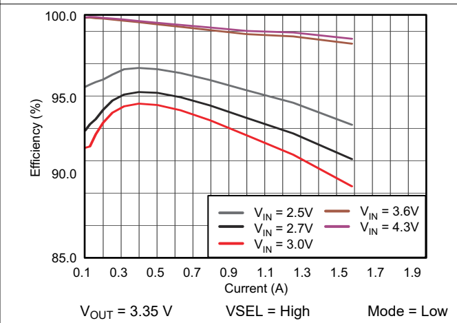
Figure 10-5. TPS61281D Efficiency vs Output Current
