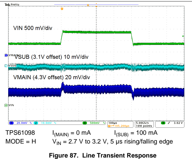
Figure 87. Line Transient Response
