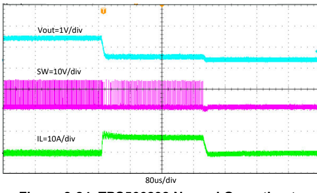
Figure 8-24. TPS566238 Normal Operation to Output Hard Short
