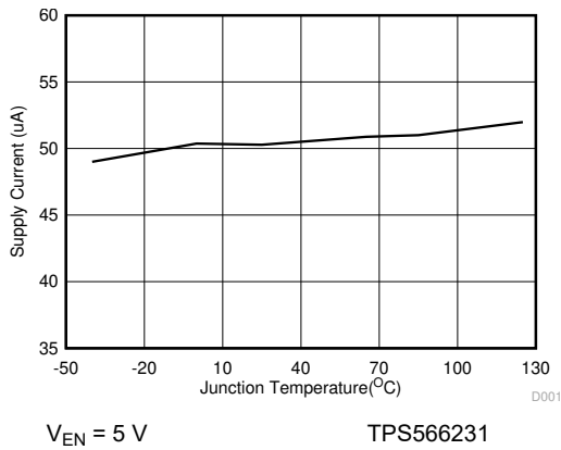
Figure 6-1. Supply Current vs Junction Temperature
