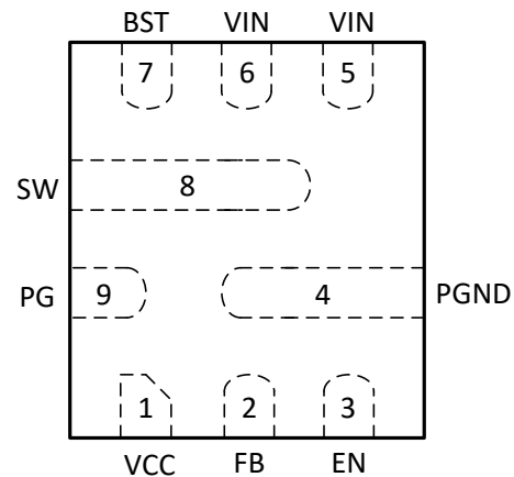
Figure 5-2. TPS566231P/TPS566238P Package (Top View)
