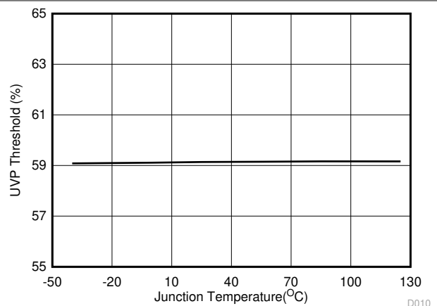
Figure 6-12. UVP Threshold vs Junction Temperature
