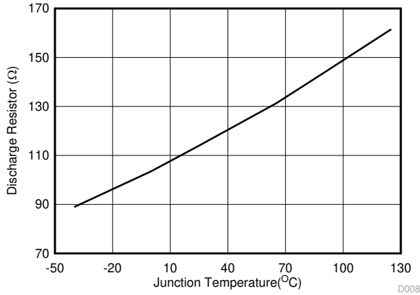
Figure 6-13. Discharge Resistor vs Junction Temperature
