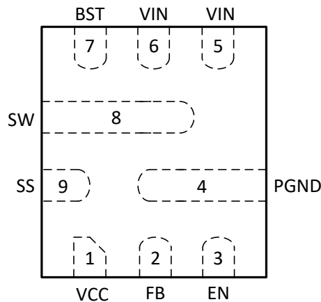
Figure 5-1. TPS566231/TPS566238 Package (Top View)
