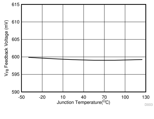
Figure 6-4. Feedback Voltage vs Junction Temperature
