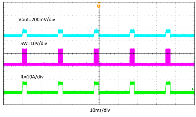
Figure 8-25. Output Hard Short Hiccup
