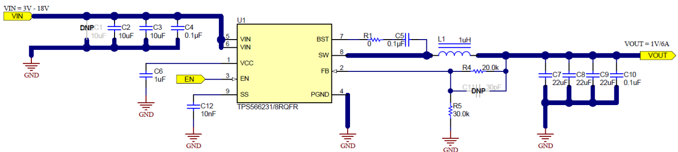
Figure 8-1. 1-V, 6-A Reference Design
