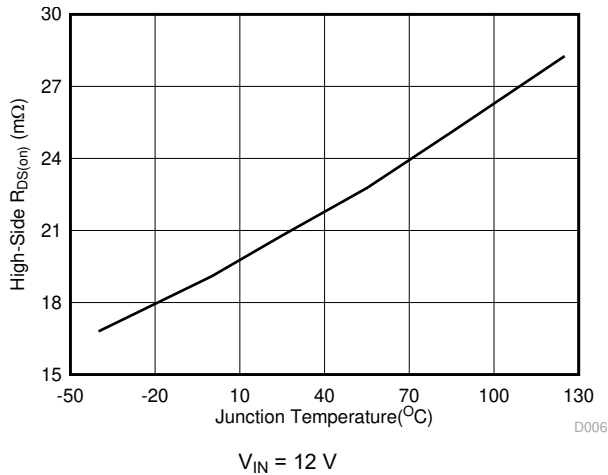
Figure 6-7. High-Side R_{DS(on)} vs Junction Temperature
