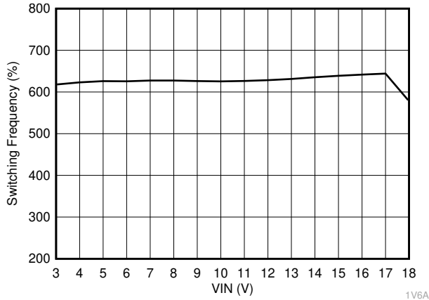
Figure 8-8. Switching Frequency vs Input Voltage
