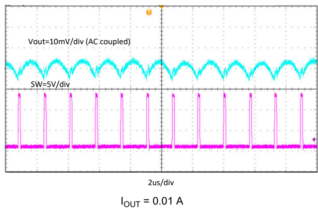
Figure 8-13. TPS566238 Output Voltage Ripple
