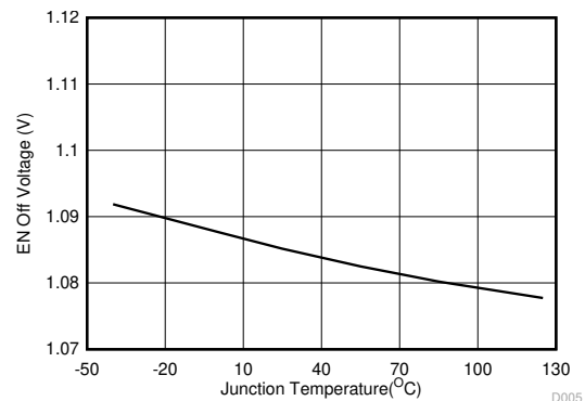
Figure 6-6. Enable Off Voltage vs Junction Temperature
