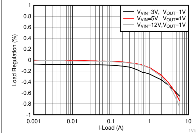
Figure 8-4. TPS566231 Load Regulation
