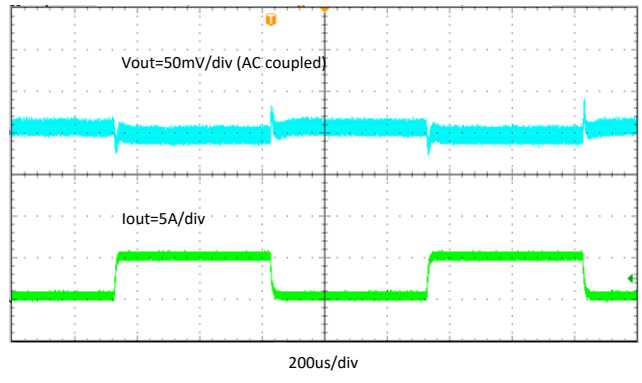
Figure 8-21. TPS566238 Transient Response
