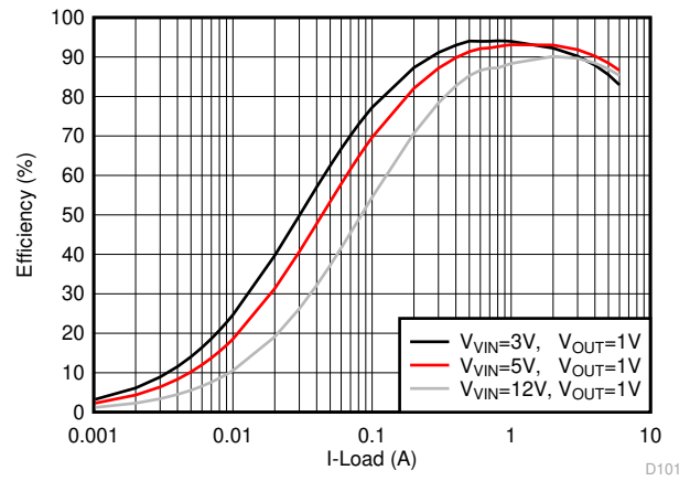
Figure 8-3. TPS566238 Efficiency Curve
