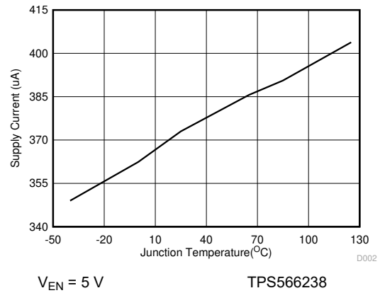
Figure 6-2. Supply Current vs Junction Temperature
