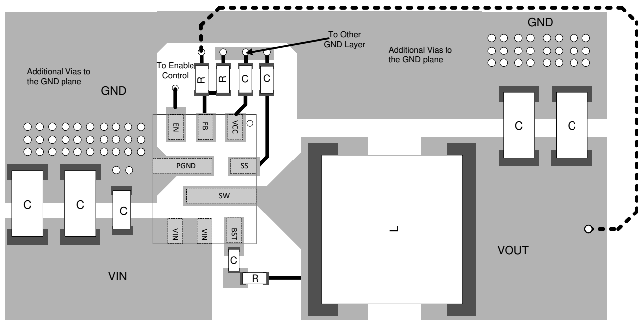
Figure 10-1. Top-Layer Layout
