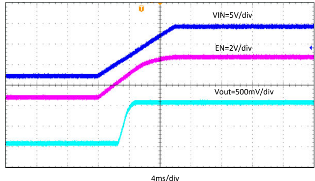
Figure 8-17. Start-up with V_{IN} Rising, I_{OUT} = 3\text{ A}
