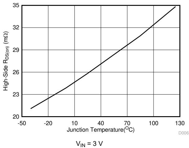
Figure 6-9. High-Side R_{DS(on)} vs Junction Temperature
