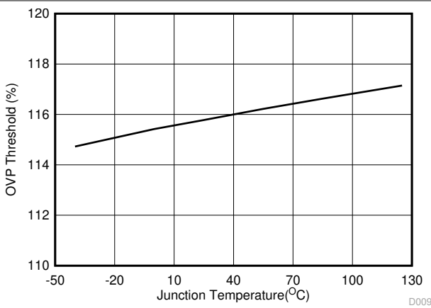
Figure 6-11. OVP Threshold vs Junction Temperature
