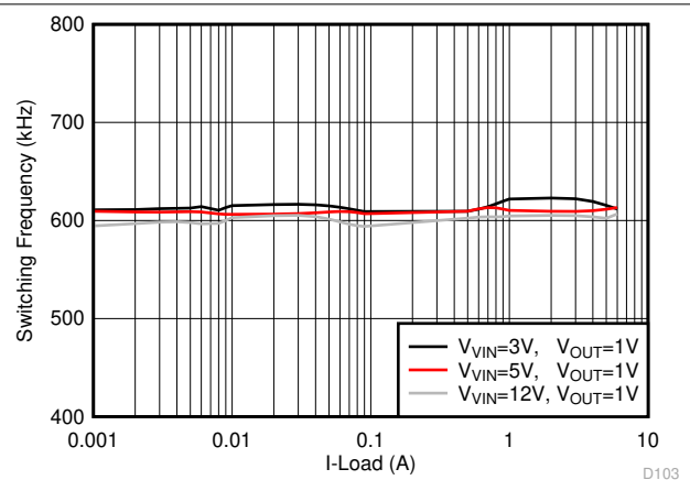
Figure 8-7. TPS566238 F_{sw} vs Output Load
