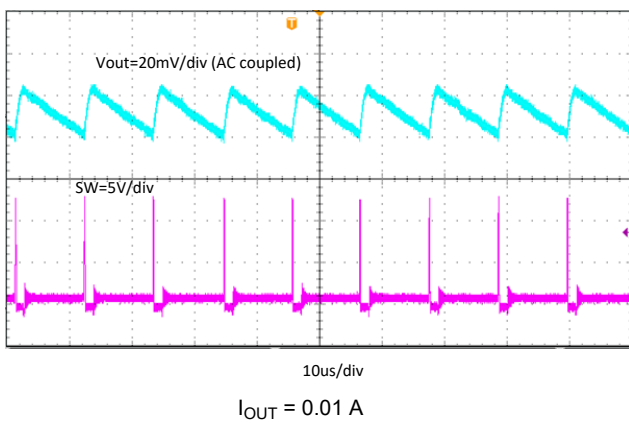
Figure 8-12. TPS566231 Output Voltage Ripple
