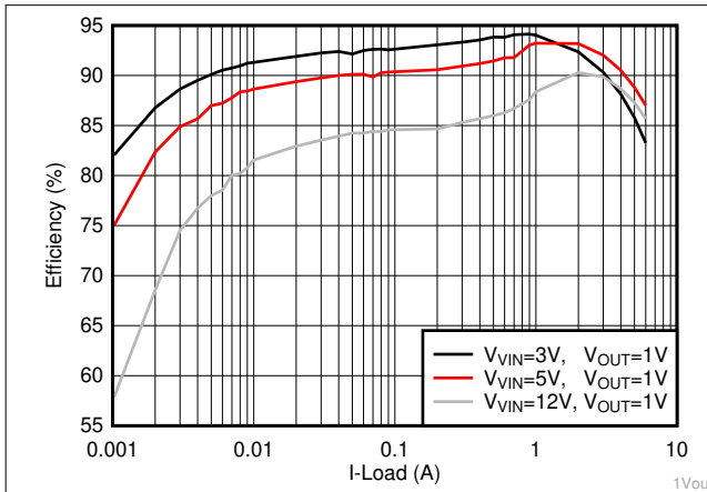
Figure 8-2. TPS566231 Efficiency Curve
