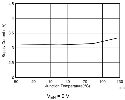
Figure 6-3. Shutdown Current vs Temperature
