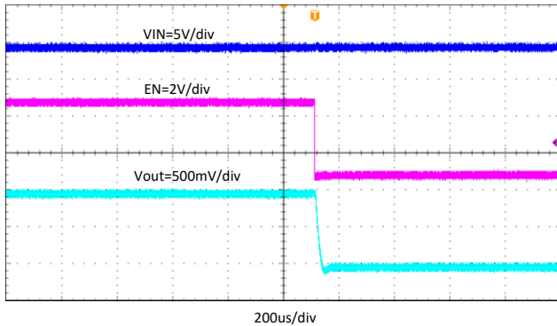
Figure 8-16. Shut-down Through EN, I_{OUT} = 3\text{ A}
