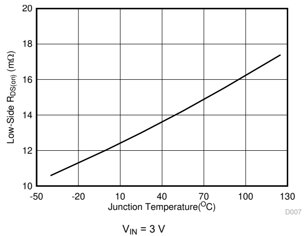
Figure 6-10. Low-Side R_{DS(on)} vs Junction Temperature
