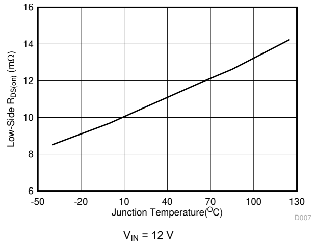
Figure 6-8. Low-Side R_{DS(on)} vs Junction Temperature
