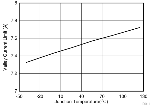
Figure 6-14. Valley Current Limit vs Junction Temperature
