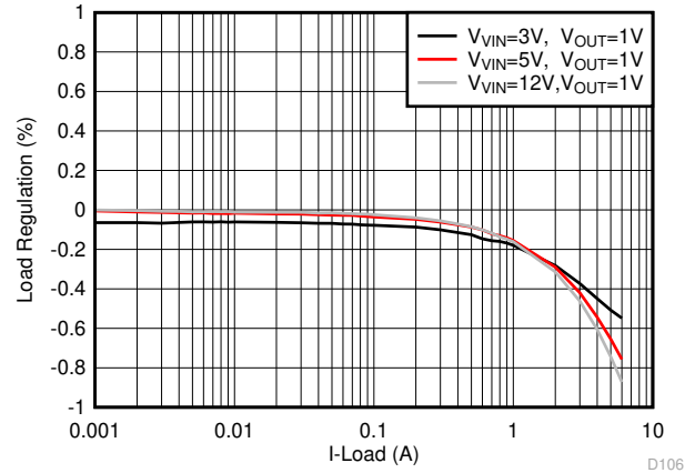
Figure 8-5. TPS566238 Load Regulation
