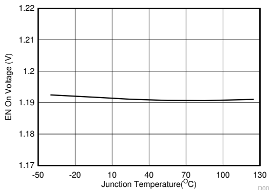
Figure 6-5. Enable On Voltage vs Junction Temperature
