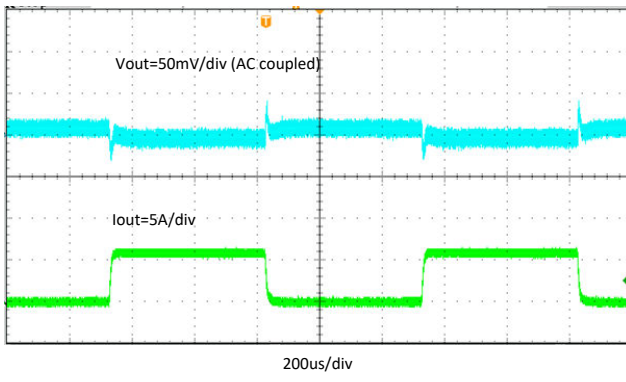
Figure 8-20. TPS566231 Transient Response
