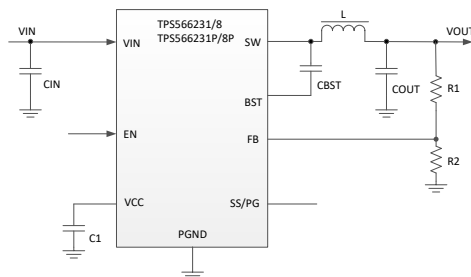
Typical Application
