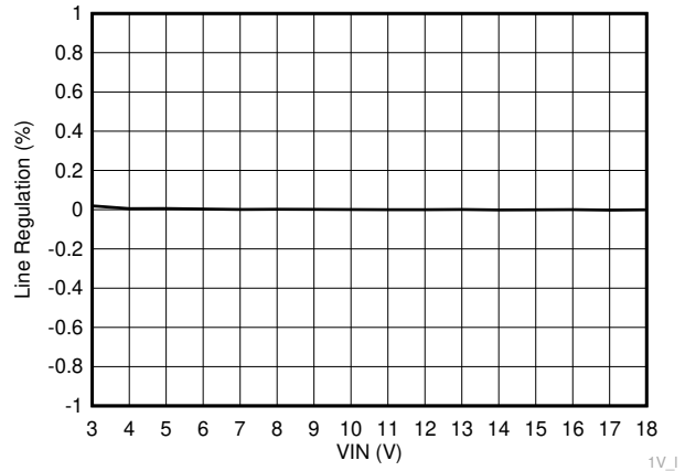
Figure 8-9. TPS566231 Line Regulation
