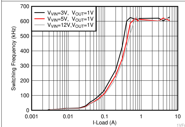
Figure 8-6. TPS566231 F_{sw} vs Output Load
