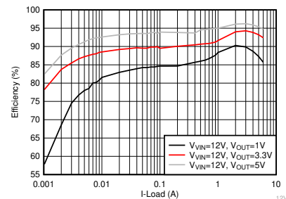
TPS566231 Efficiency Versus Output Current
