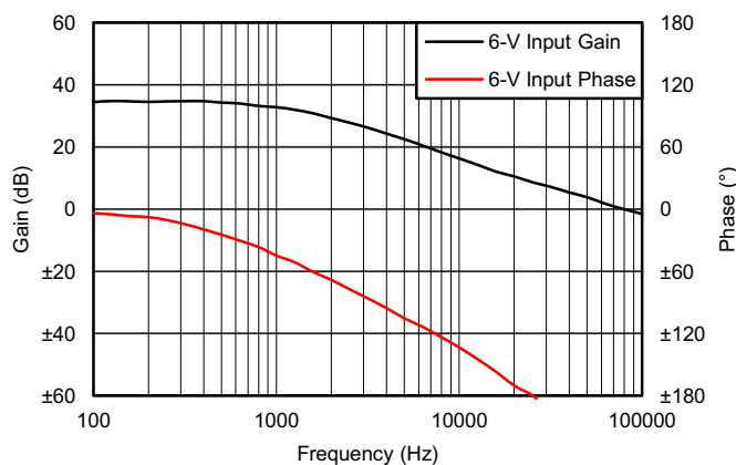
Figure 27. SEPIC Power Stage Gain and Phase
