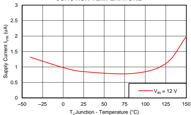
SHUTDOWN SUPPLY CURRENT VS JUNCTION TEMPERATURE
