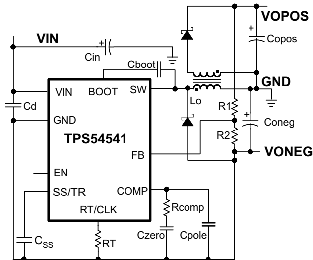
Figure 73. TPS54541 Split Rail Power Supply Based on the Application Note, SLVA369
