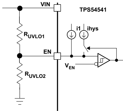
Figure 26. Adjustable Undervoltage Lockout (UVLO)
