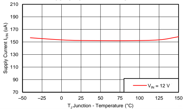
V_IN SUPPLY CURRENT VS JUNCTION TEMPERATURE
