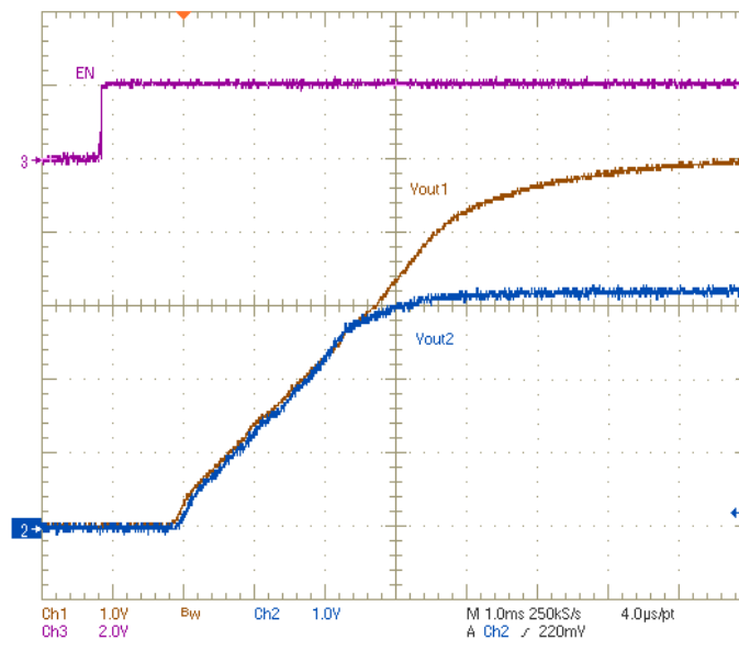
Figure 36. Simultaneous Startup With Tracking Resistor
