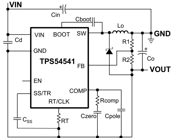
Figure 72. TPS54541 Inverting Power Supply Based on the Application Note, SLVA317
