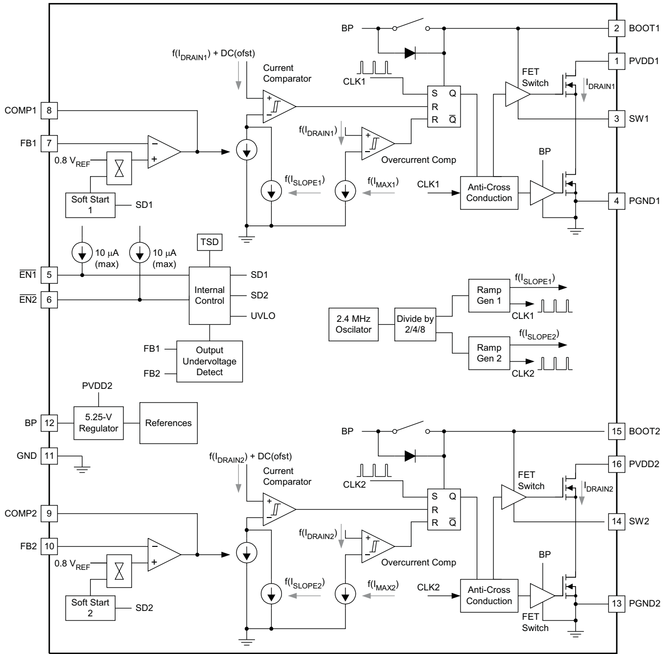
Figure 11. Block Diagram
