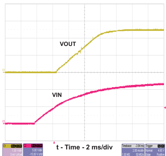
Figure 23. TPS54232 Start Up
