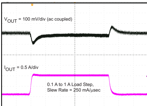
Time - 200 μs/div
