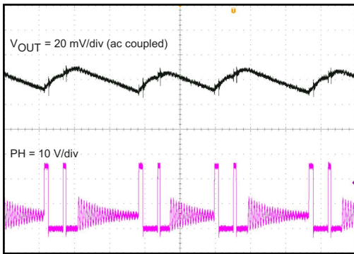
Time - 4 μs/div
