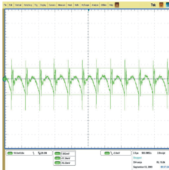
Figure 25. Output Ripple 10 mV/div, 2- \mu s/div, 20-MHz Bandwidth
