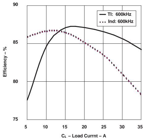
Figure 34. Efficiency vs. Load Current
