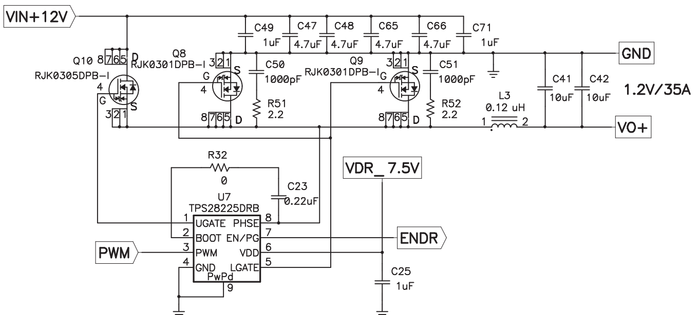
Figure 31. One of Four Phases Driven by TPS28225-Q1 Driver in 4-phase VRM Reference Design
