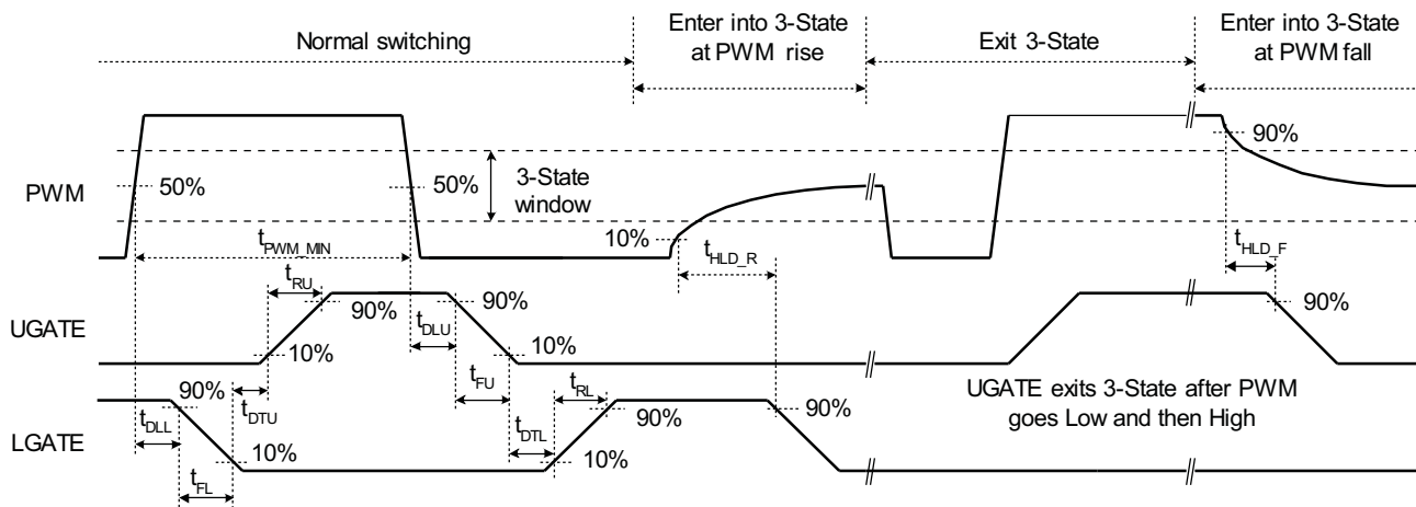
Figure 1. TPS28225-Q1 Timing Diagram
