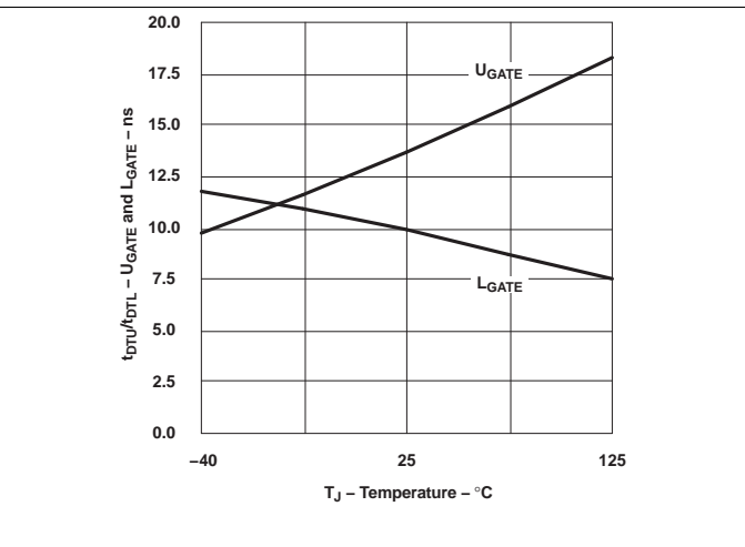
Figure 11. UGATE and LGATE (Dead Time) vs. Temperature ( V_{DD} = 7.2\text{ V} , C_{LOAD} = 3\text{ nF} )
