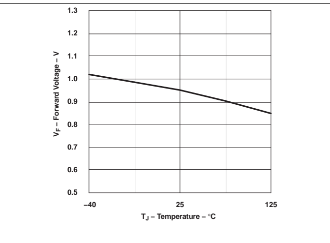
Figure 13. Bootstrap Diode Forward Voltage vs. Temperature ( V_{DD} = 7.2\text{ V} , I_F = 100\text{ mA} )
