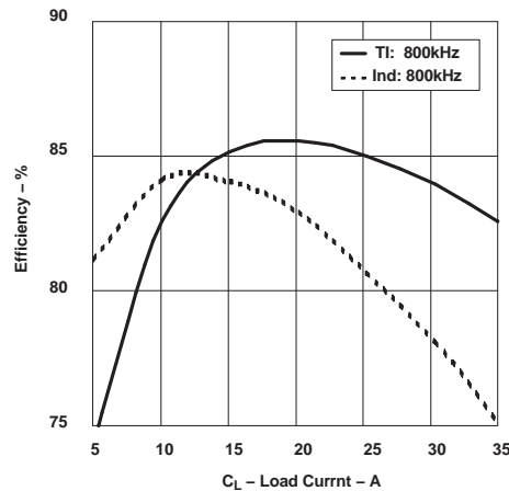
Figure 36. Efficiency vs. Load Current
