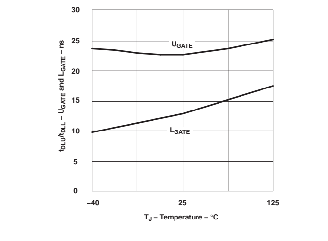
Figure 10. UGATE and LGATE (Turning OFF Propagation Delays) vs. Temperature ( V_{DD} = 7.2\text{ V} , C_{LOAD} = 3\text{ nF} )
