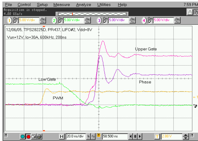
Figure 39. Phase Rising Edge Switching Waveforms (20 ns/div) of the Power Stage in Figure 31
