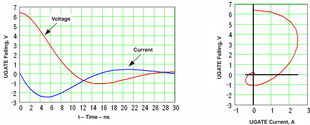
Figure 27. UGATE Turning Off Voltage and Sink Current vs Time (Related Switching Diagram (right))
