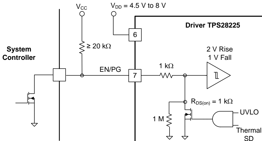
Figure 20. Enable/Power Good Circuit
