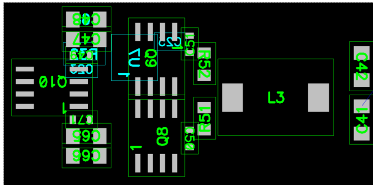
Figure 41. Component Placement Based on Schematic in Figure 31
