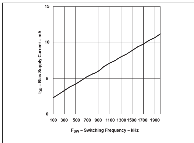
Figure 14. Bias Supply Current vs. Switching Frequency ( V_{DD} = 7.2\text{ V} , No Load, T_J = 25^\circ\text{C} )
