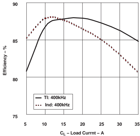
Figure 32. Efficiency vs. Load Current
