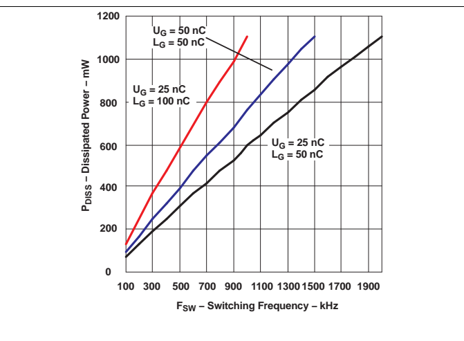
Figure 15. Driver Dissipated Power vs. Switching Frequency (Different Load Charge, V_{DD} = 7.2\text{ V} , T_J = 25^\circ\text{C} )
