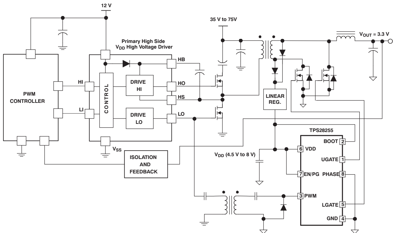
Figure 29. Driver for Synchronous Rectification with Complementary Driven MOSFETs
