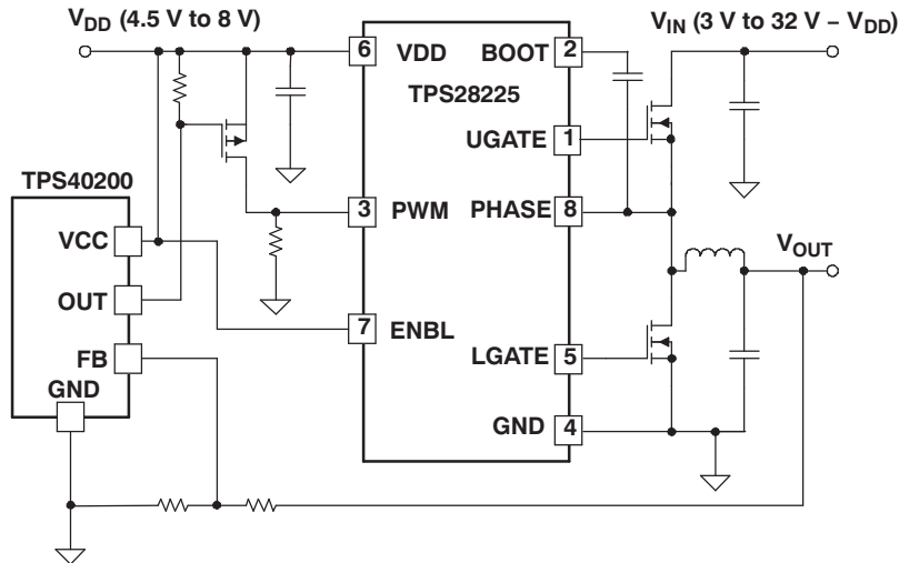
Figure 28. One-Phase POL Regulator
