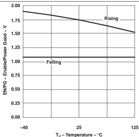
Figure 4. Enable/Power Good Threshold vs. Temperature ( V_{DD} = 7.2\text{ V} )
