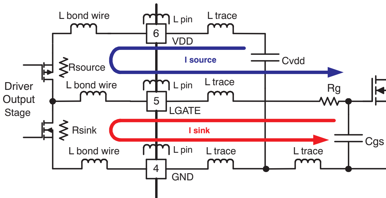
Figure 25. MOSFET Drive Paths and Main Circuit Parasitics
