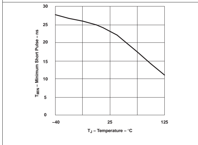
Figure 12. UGATE Minimum Short Pulse vs. Temperature ( V_{DD} = 7.2\text{ V} , C_{LOAD} = 3\text{ nF} )
