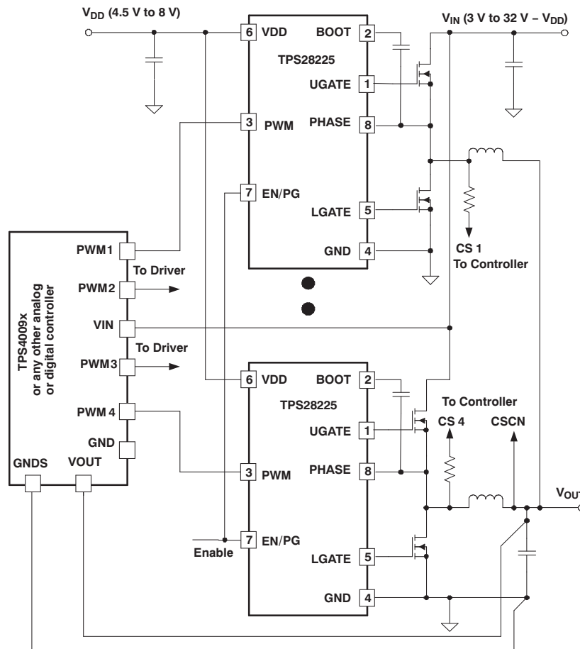
Figure 30. Multi-Phase Synchronous Buck Converter
