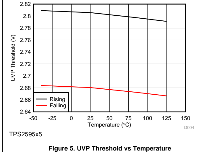
Figure 5. UVP Threshold vs Temperature
