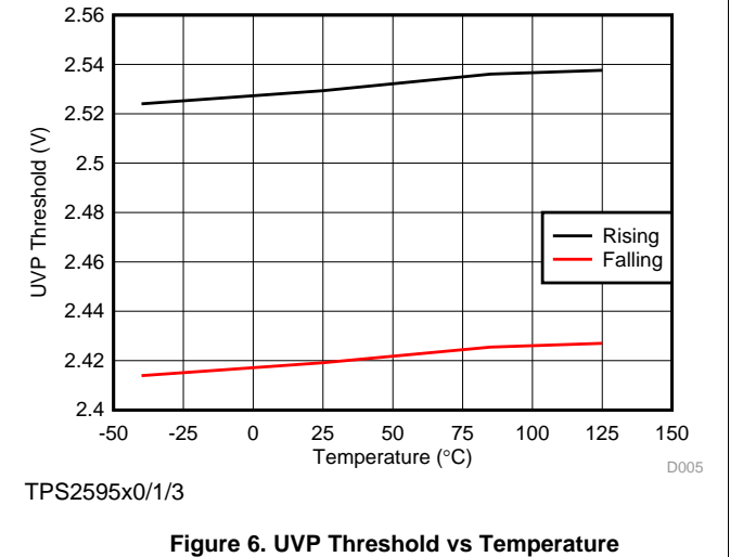
Figure 6. UVP Threshold vs Temperature
