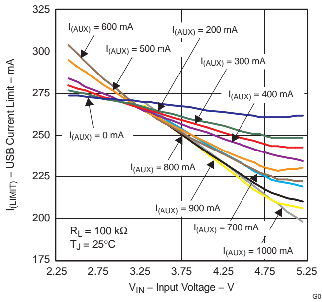
Figure 19. USB Current-Limit Threshold vs V_{IN} , R_{LIM} = 100\text{ k}\Omega , T_A = 25\text{ }^\circ\text{C}
