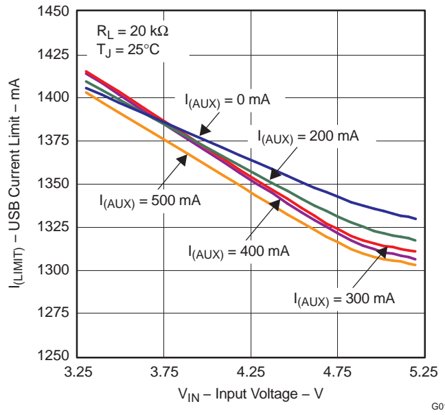
Figure 17. USB Current-Limit Threshold vs V_{IN} , R_{LIM} = 20\text{ k}\Omega , T_A = 25\text{ }^\circ\text{C}
