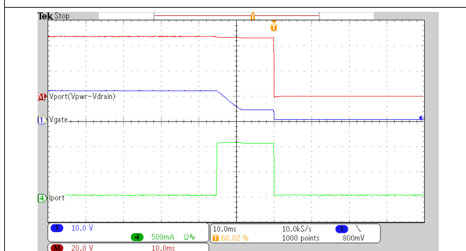
Figure 86. Response to a 25-Ω Load - PoE+ Mode
