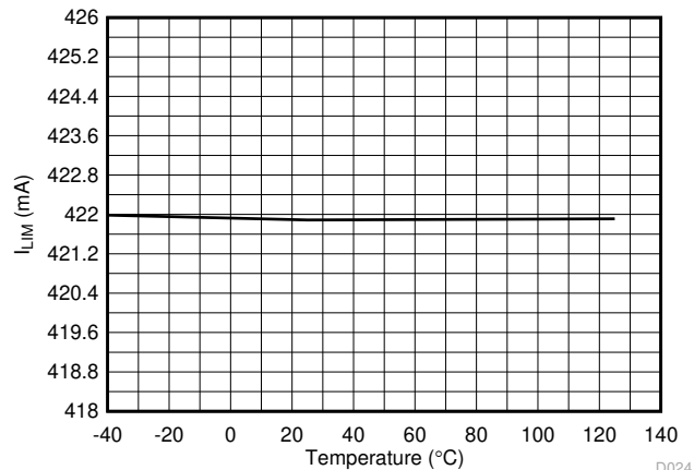
Figure 7-22. 1x Mode ( 2x\text{FBn} = 0 ) Current Limit vs Temperature
