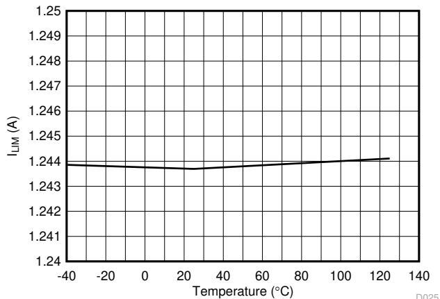
Figure 7-23. 2x Mode ( 2x\text{FBn} = 1 ) Current Limit vs Temperature
