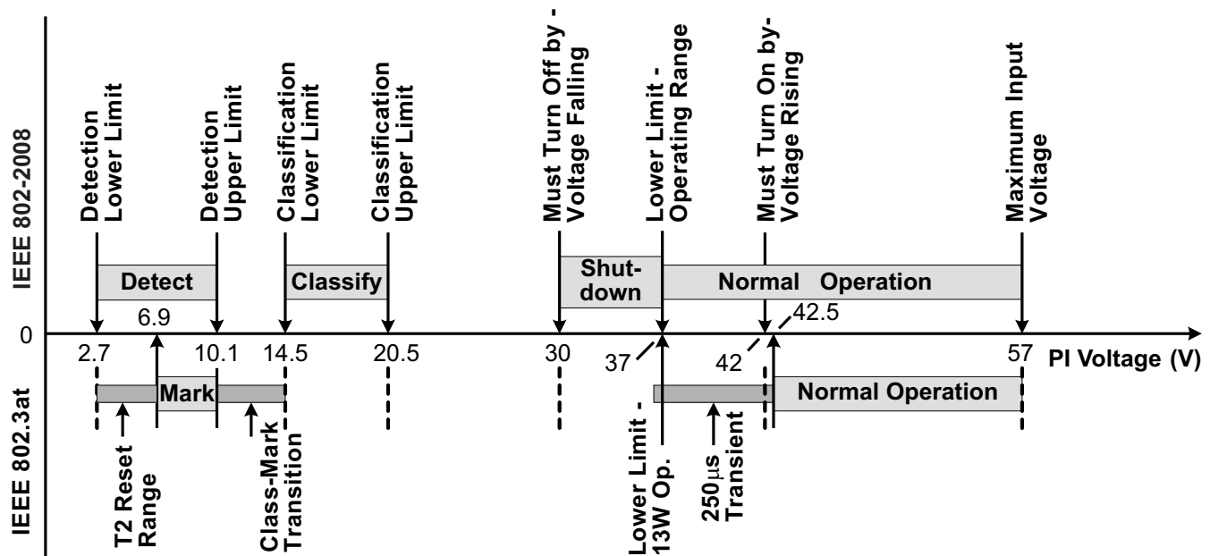
Figure 18. Threshold Voltages
