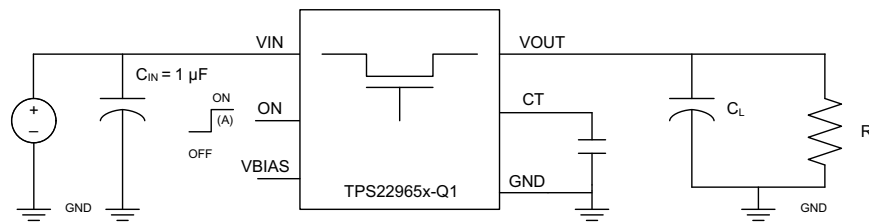
Figure 1. Test Circuit
