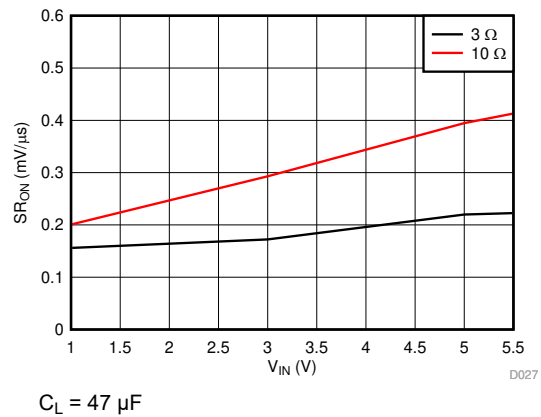
Figure 7-24. Slew Rate vs Load Resistance (CT = 10000 pF)
