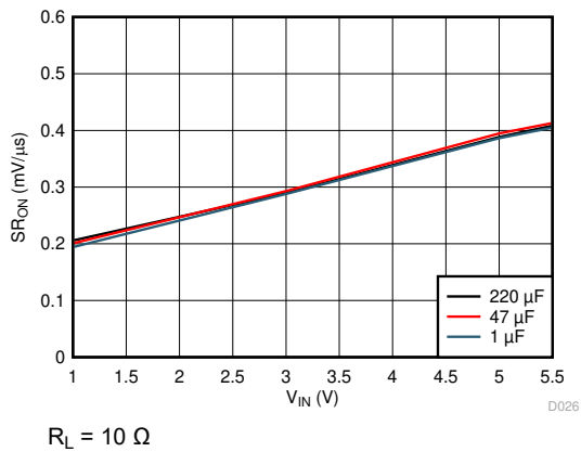
Figure 7-23. Slew Rate vs Load Capacitance (CT = 10000 pF)
