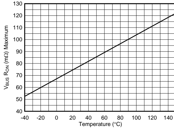
Figure 29. TPD3S716-Q1 Maximum V_{BUS} R_{ON} vs. Junction Temperature
