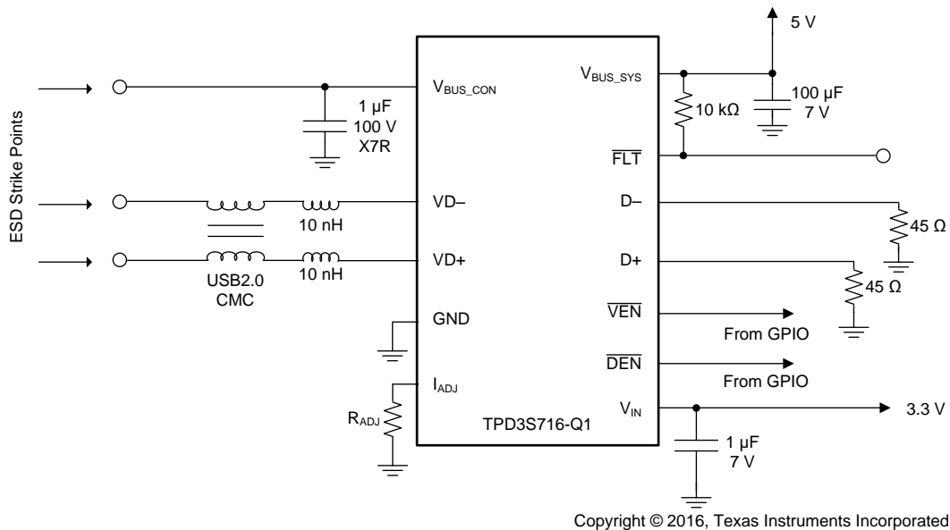
Figure 20. ESD System Test Setup
