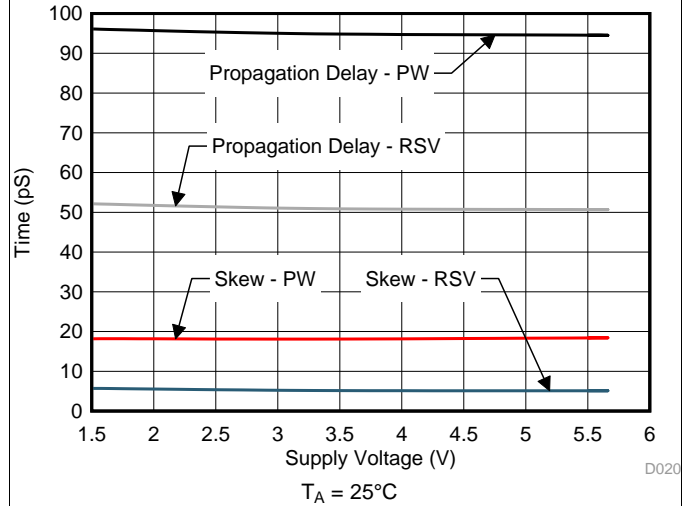
Figure 20. Skew and Propagation Delay vs Supply Voltage
