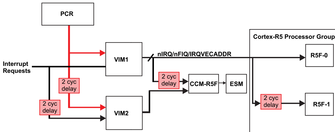
Figure 6-17. Interrupt Generation
