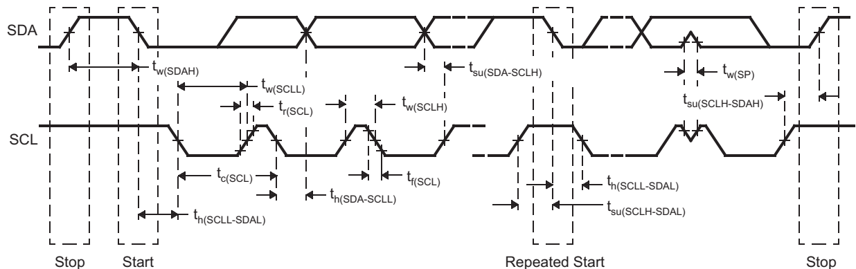
Figure 7-18. I2C Timings
