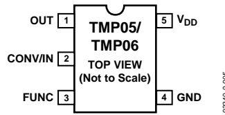
Figure 5. Pin Configuration
