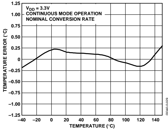
Figure 15. Output Accuracy vs. Temperature
