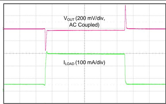
Time (20 \mu\text{s}/\text{div} ) V_{IN} = 2.0\text{ V} , no output capacitor, output current slew rate = 0.25\text{ A}/\mu\text{s}
