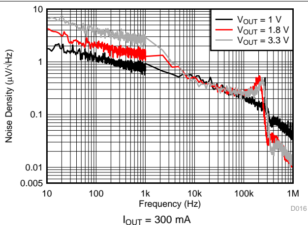
Figure 10. Output Spectral Noise Density vs Frequency and Output Voltage
