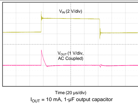
Figure 11. Line Transient
