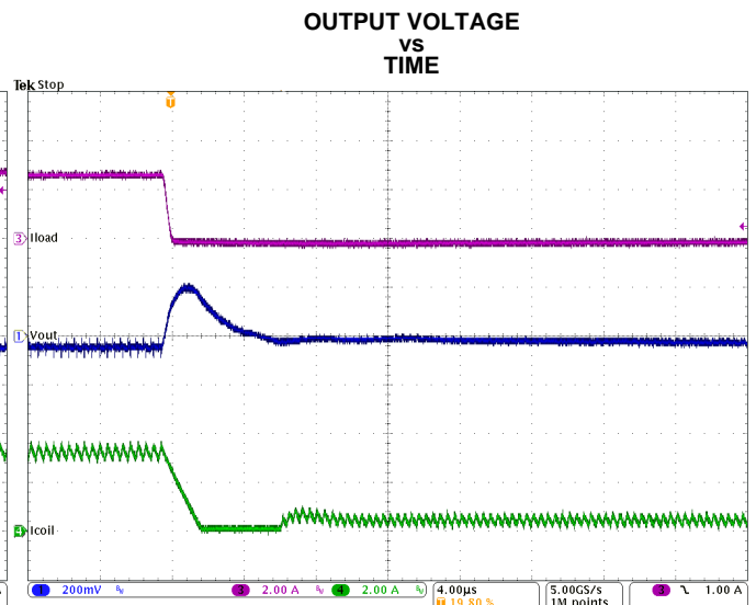
Figure 31. Load Transient Response of Figure 29, falling edge
