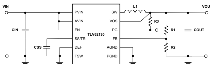
Figure 3. Measurement Setup
